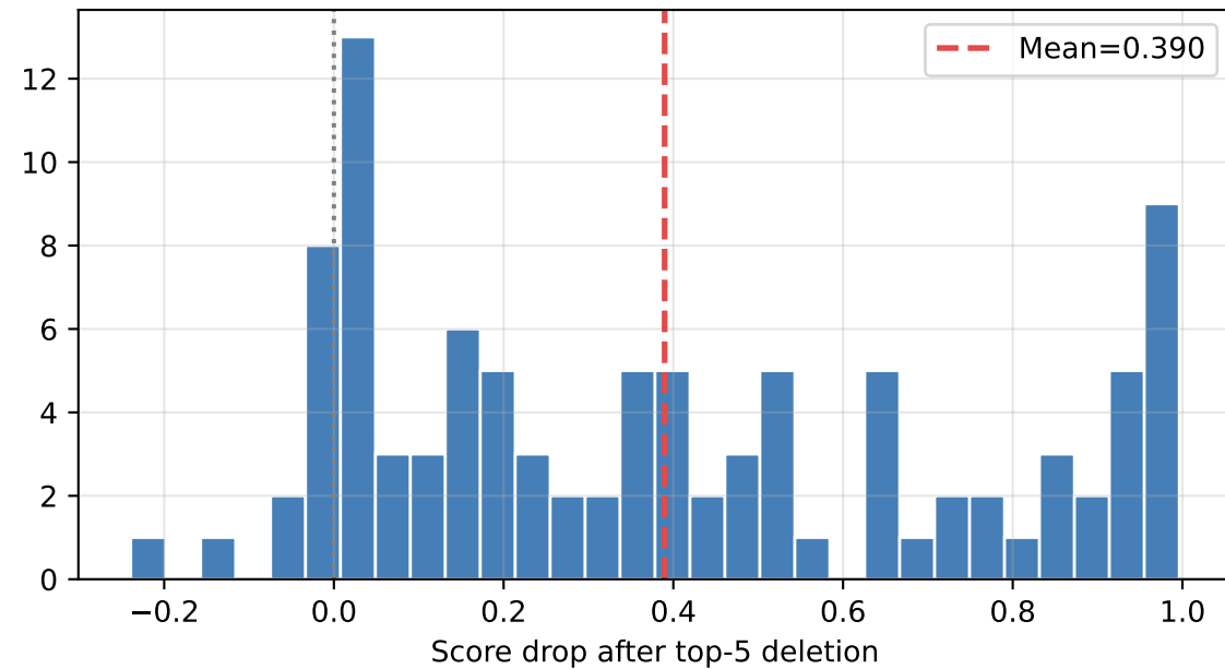
Faithfulness: deletion test
