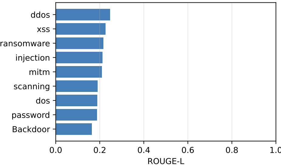
ROUGE-L per Attack Class
