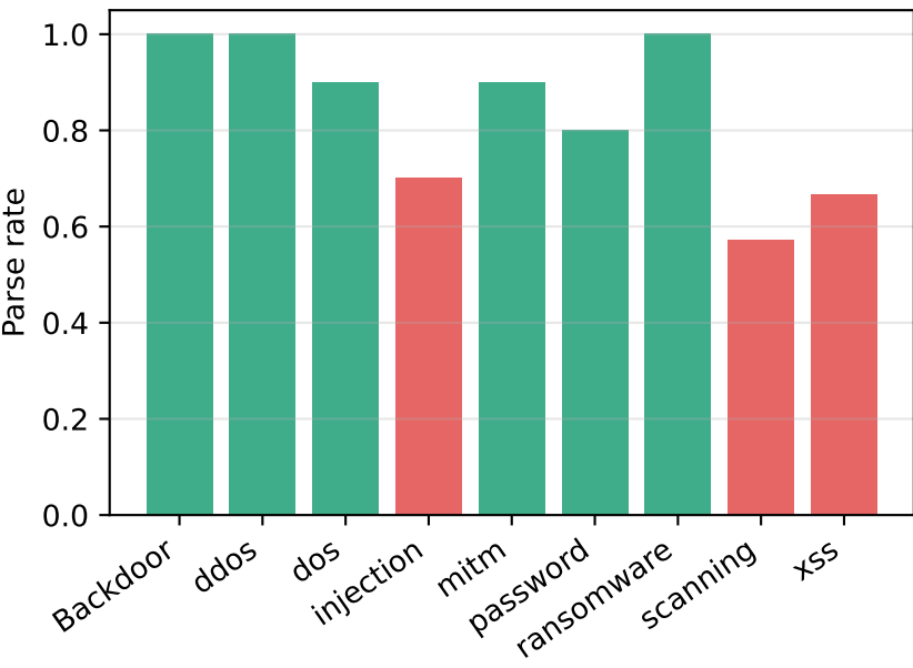
JSON Parse Success Rate per Class
