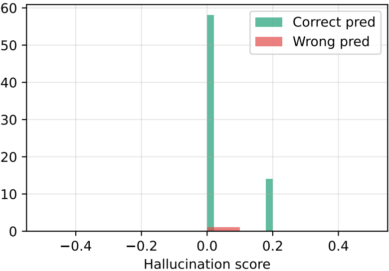
Hallucination: Correct vs Wrong Predictions
