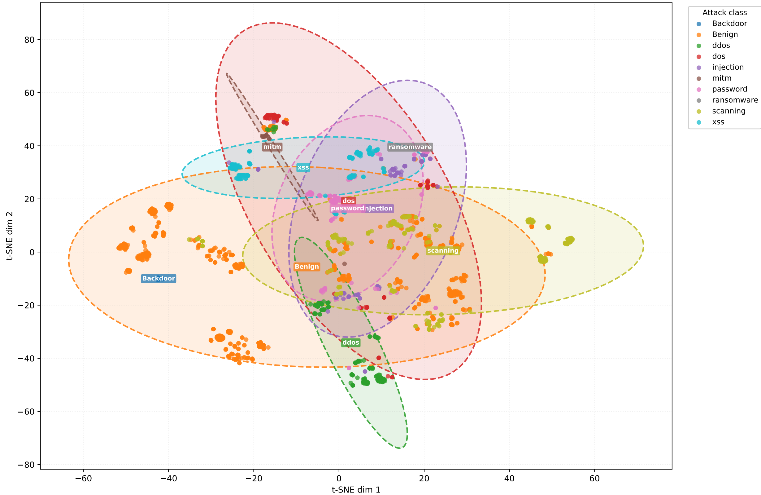
t-SNE of Retrieval Embeddings — Test Set (ellipses = 2- \sigma confidence region per class)
