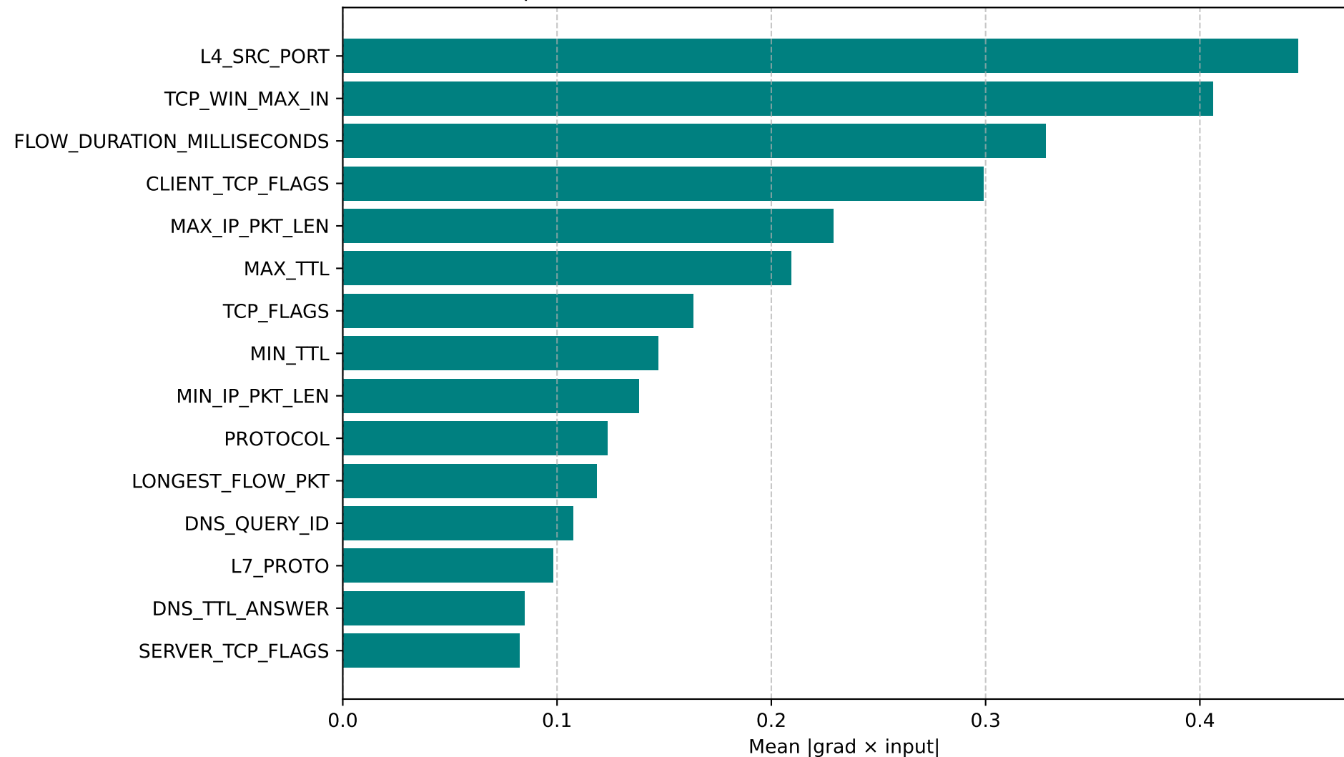
Top 15 Most Influential NetFlow Features (Global Attribution)
