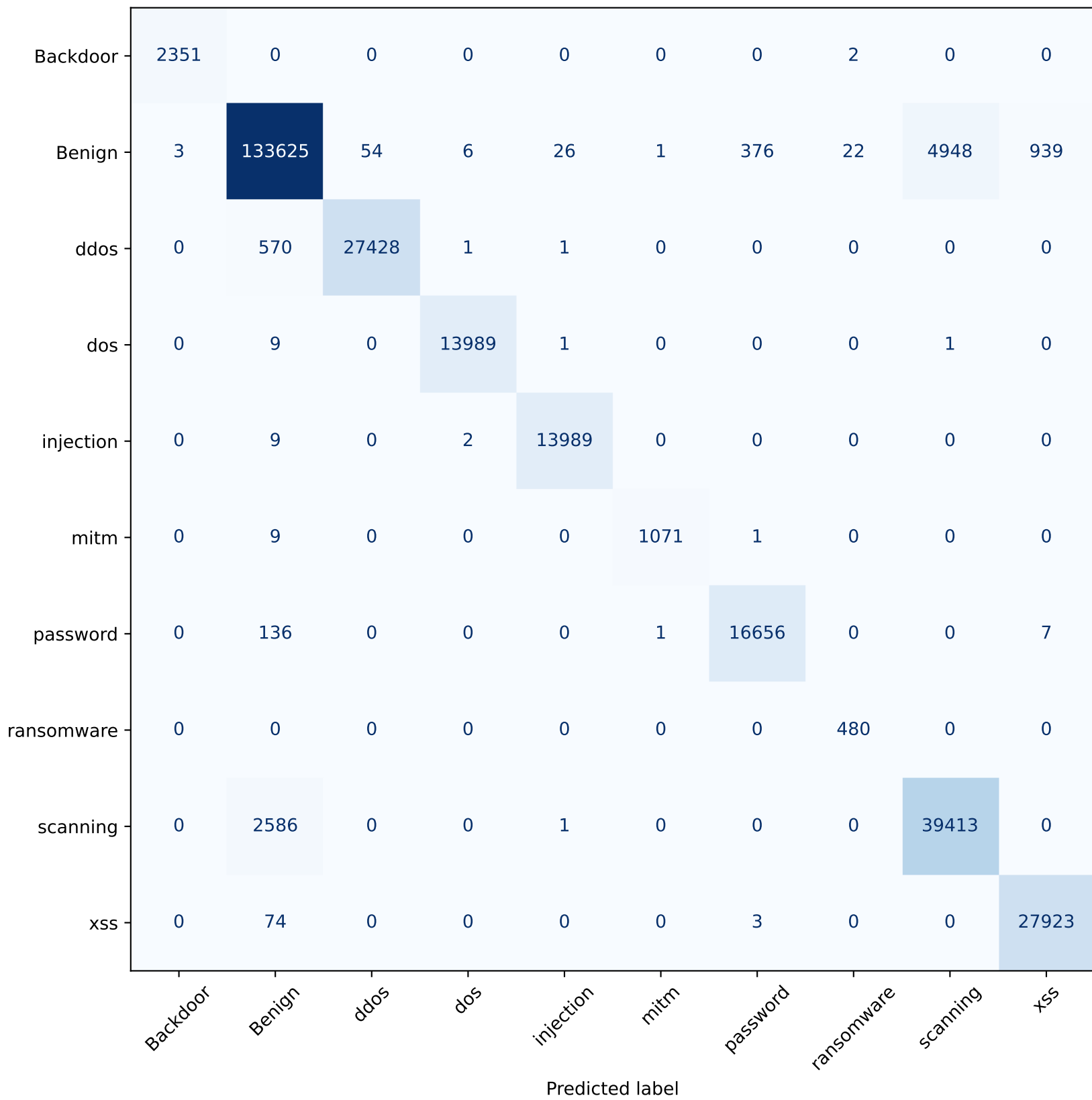
Confusion Matrix — Test Set
