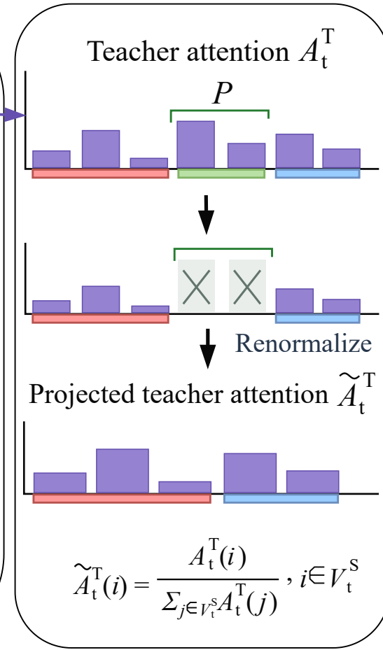
3. Student-Support Projection
