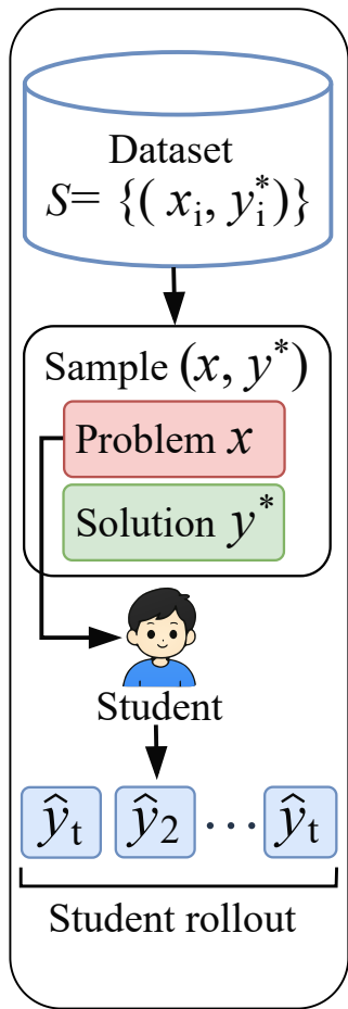
1. On-Policy Sampling
