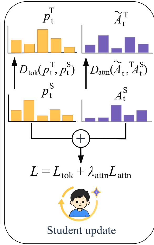
4. Joint Distillation
