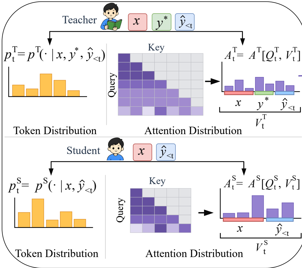
2. Teacher-Student Distributions
