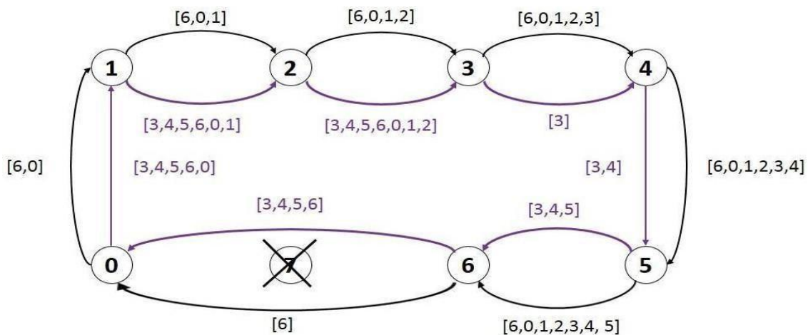
Figure 2: Ring Algorithm
