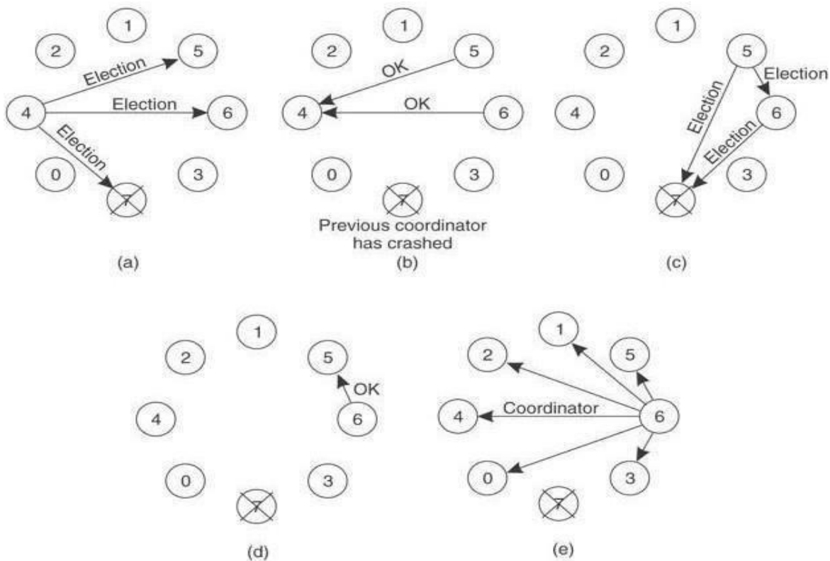
Figure 1: Bully Algorithm
