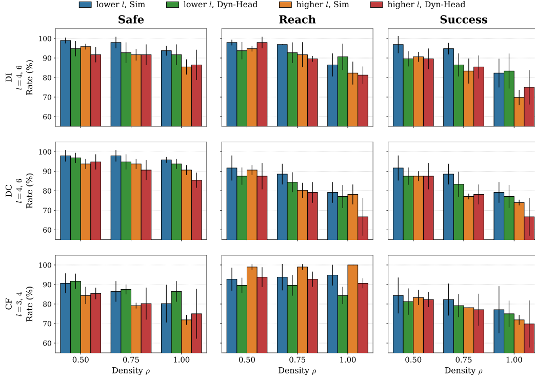
Figure 2: Zero-shot generalization across obstacle densities \rho = M/l^{n_p} and workspace sizes. Rows show DI, DC, and CF; columns show safe, reach, and success rates. Colors distinguish Sim and Dyn-Head at the smaller and larger workspace sizes. Bars report mean \pm standard deviation over 32 environments and 3 seeds. Models are trained only at \rho = 0.50 and the smaller workspace size.
