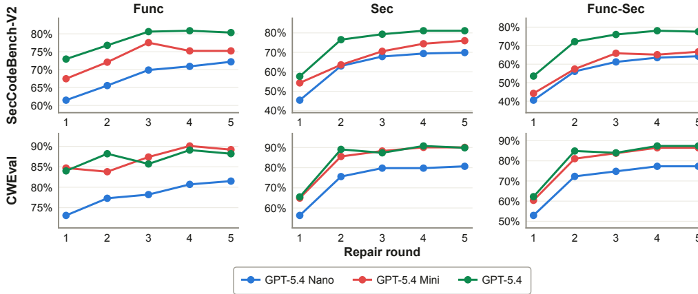
Figure 6: Per-round repair with FALCON feedback on SecCodeBench-V2 (top) and CWEval (bottom), reporting functional correctness (Func), security (Sec), and their joint rate (Func-Sec). Across all models, security and Func-Sec rise sharply in the first two rounds and then plateau, while functional correctness is maintained or improved.
