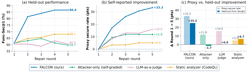
Figure 3: Repair loop on CWEval with four security feedback signals and GPT-5.4-MINI as the coding model. (left) Held-out Func-Sec@1, graded by CWEval’s ground-truth tests, which no signal observes. (middle) Proxy secure rate, the improvement each signal reports on its own verdicts, relative to round one. (right) Reported versus held-out improvement from round one to five. FALCON produces the largest held-out improvement. CodeQL transfers a smaller gain, while the LLM-as-a-judge and attacker-only signals almost do not transfer.
