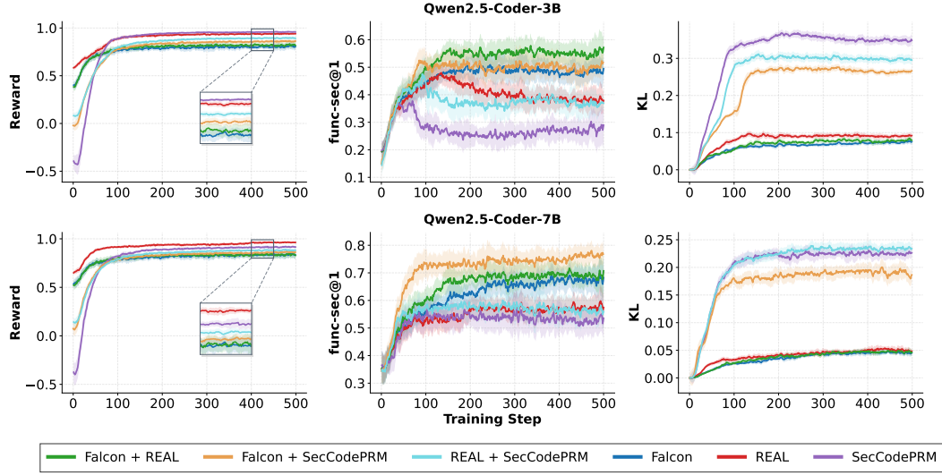
Figure 5: FALCON provides a robust RL signal and strengthens existing security rewards. Every policy steadily increases its own training reward (left), yet held-out Func-Sec@1 separates sharply (middle). When optimized alone, REAL (Yao et al., 2025) and SecCodePRM (Yu et al., 2026) transfer much less of their reward gains to held-out Func-Sec@1, most clearly at 3B, where Func-Sec@1 eventually declines while training reward keeps increasing, consistent with reward overoptimization. In contrast, FALCON maintains stronger held-out Func-Sec@1, and combining it with either reward further improves transfer, whereas combining REAL and SecCodePRM does not. Configurations that include FALCON also keep KL lower (right).
