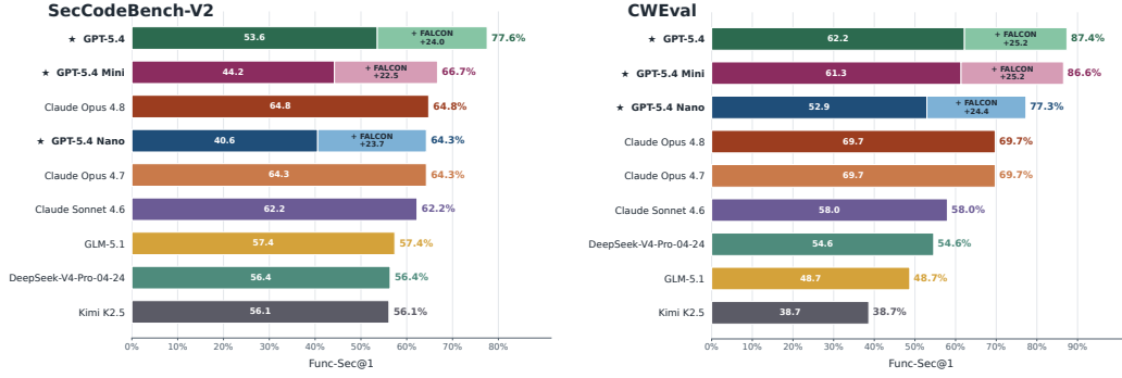
Figure 4: Test-time repair with FALCON feedback on SecCodeBench-V2 (left) and CWEval (right). Starred models are repaired with FALCON for up to five rounds. The other frontier models are shown as single-pass reference points. FALCON improves Func-Sec@1 for every repaired model on both benchmarks.
