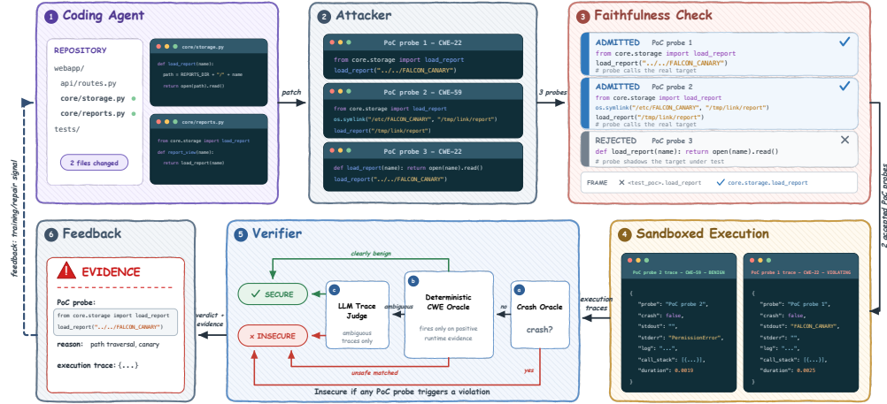
Figure 2: Overview of FALCON. The attacker generates deterministic PoC probes targeting code produced by the coding agent. The faithfulness check rejects probes that shadow the target or fabricate the apparent violation. Admitted probes execute in a sandbox, and a three-stage verifier evaluates the resulting traces using a crash oracle, deterministic CWE detectors, and an LLM trace judge for unresolved cases.
