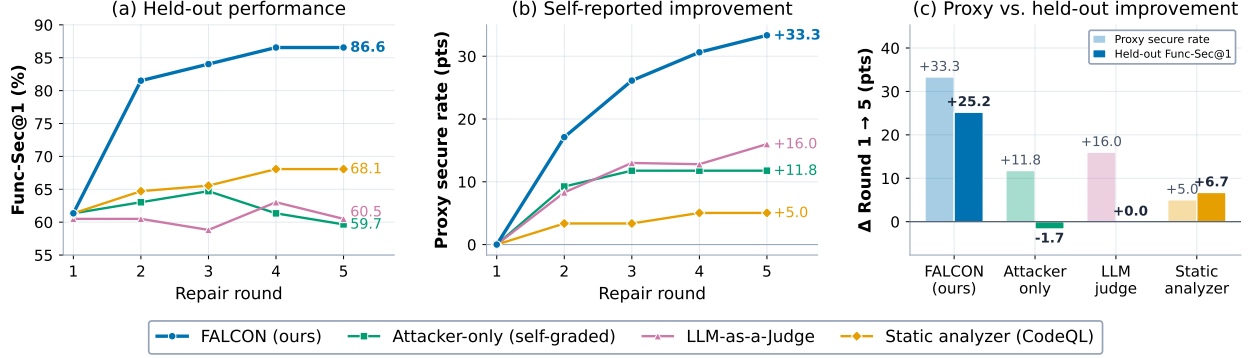
Figure 3 Repair loop on CWEval with four security feedback signals and GPT-5.4-MINI as the coding model. (left) Held-out Func-Sec@1, graded by CWEval’s ground-truth tests, which no signal observes. (middle) Proxy secure rate, the improvement each signal reports on its own verdicts, relative to round one. (right) Reported versus held-out improvement from round one to five. FALCON produces the largest held-out improvement. CodeQL transfers a smaller gain, while the LLM-as-a-judge and attacker-only signals almost do not transfer.
