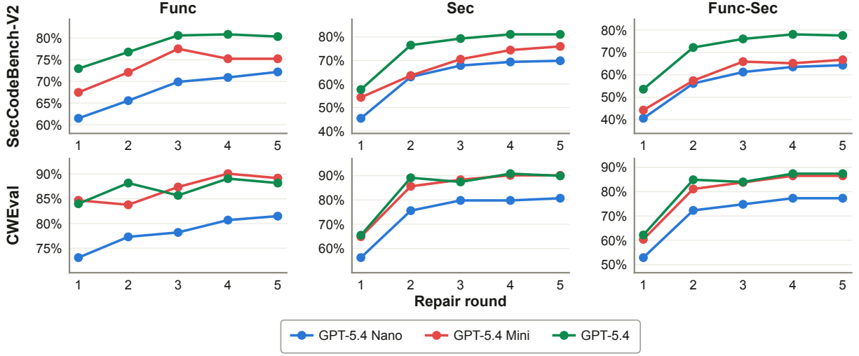
Figure 6 Per-round repair with FALCON feedback on SecCodeBench-V2 (top) and CWEval (bottom), reporting functional correctness (Func), security (Sec), and their joint rate (Func-Sec). Across all models, security and Func-Sec rise sharply in the first two rounds and then plateau, while functional correctness is maintained or improved.
