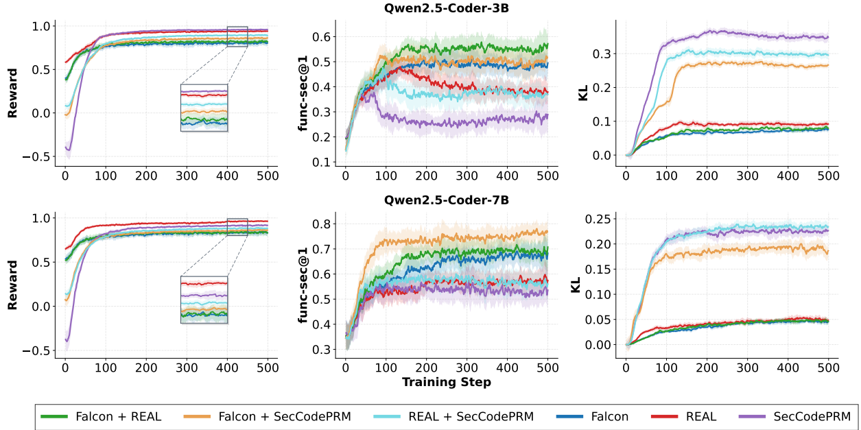
Figure 5 FALCON provides a robust RL signal and strengthens existing security rewards. Every policy steadily increases its own training reward ( left ), yet held-out Func-Sec@1 separates sharply ( middle ). When optimized alone, REAL [63] and SecCodePRM [64] transfer much less of their reward gains to held-out Func-Sec@1, most clearly at 3B, where Func-Sec@1 eventually declines while training reward keeps increasing, consistent with reward overoptimization. In contrast, FALCON maintains stronger held-out Func-Sec@1, and combining it with either reward further improves transfer, whereas combining REAL and SecCodePRM does not. Configurations that include FALCON also keep KL lower ( right ).
