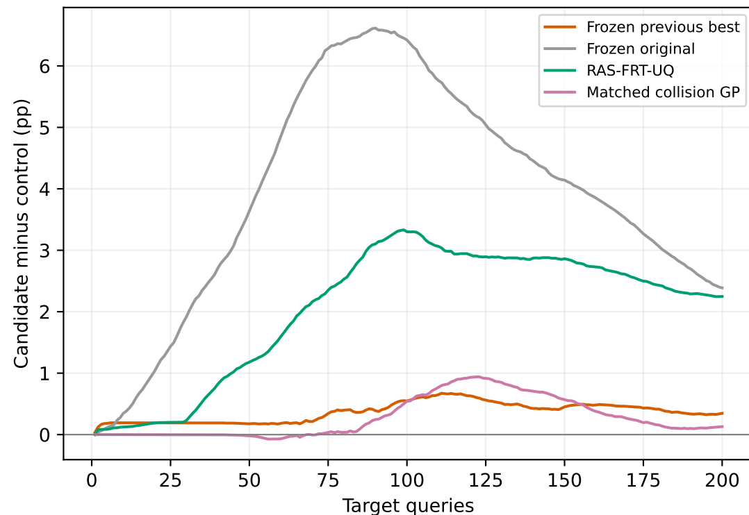
Against Matched collision GP
