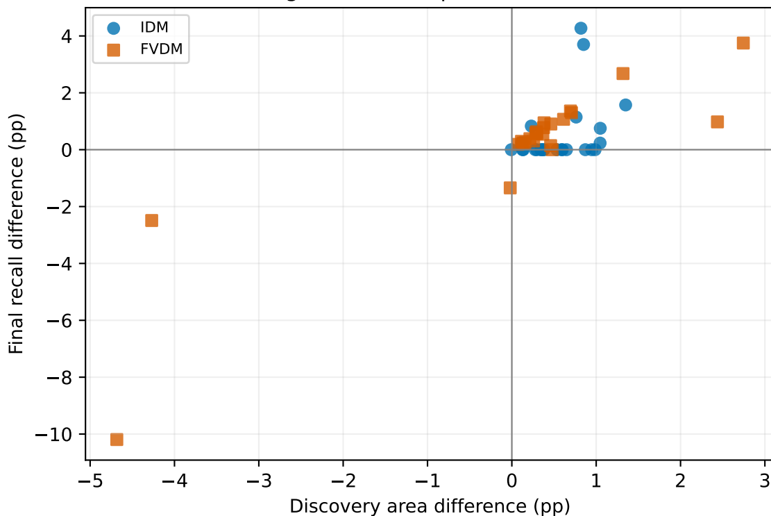
Against Frozen previous best
