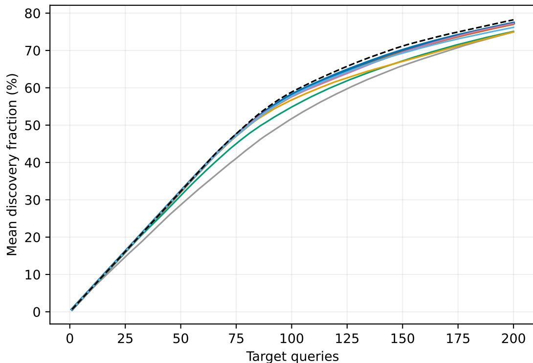
Against Frozen previous best
