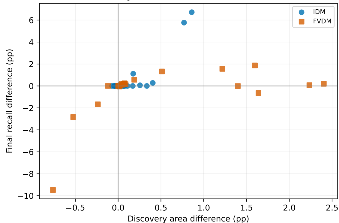
Against Matched collision GP
