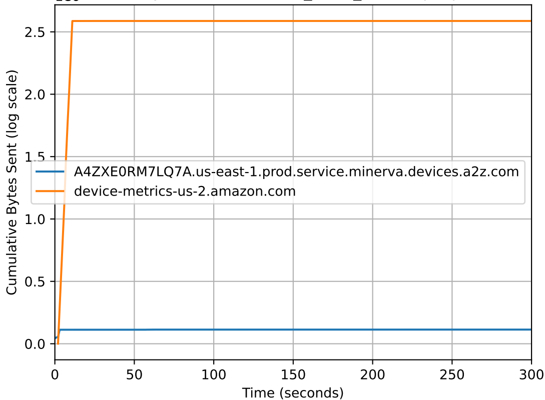
1e6 CDF of Bytes Sent for alexa_swan_kettle - pcapdroid
