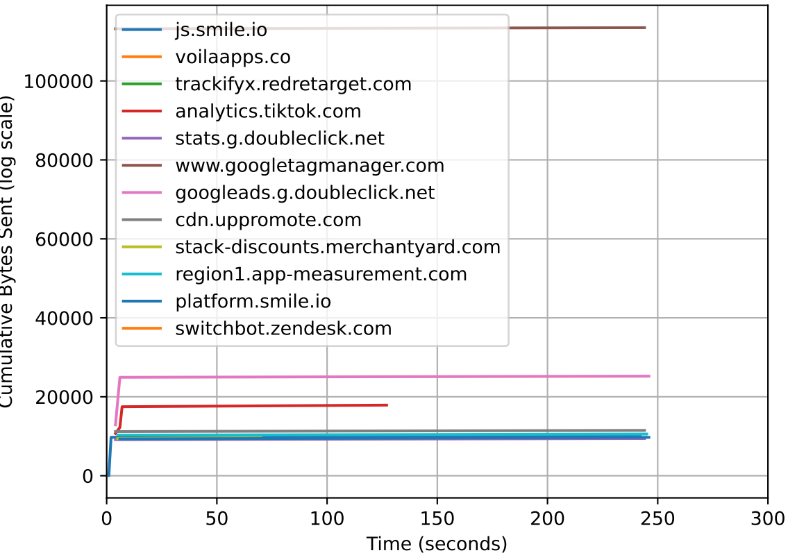
CDF of Bytes Sent for switchbot_hub_mini_1 - pcapdroid
