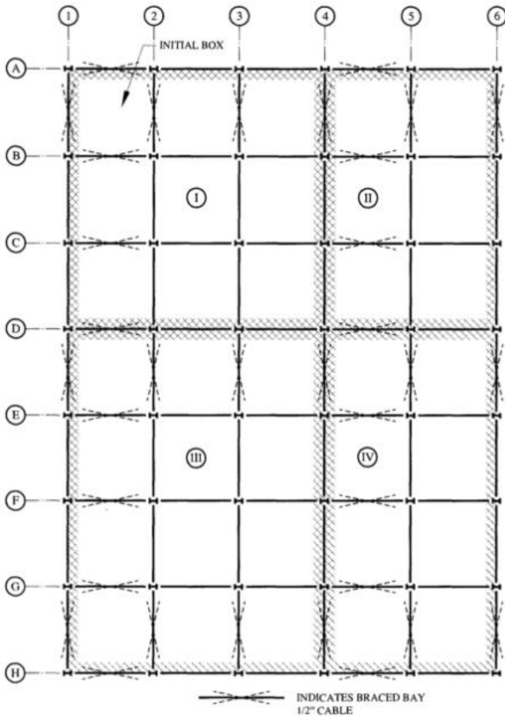
Fig. 7.1 Erection Plan
