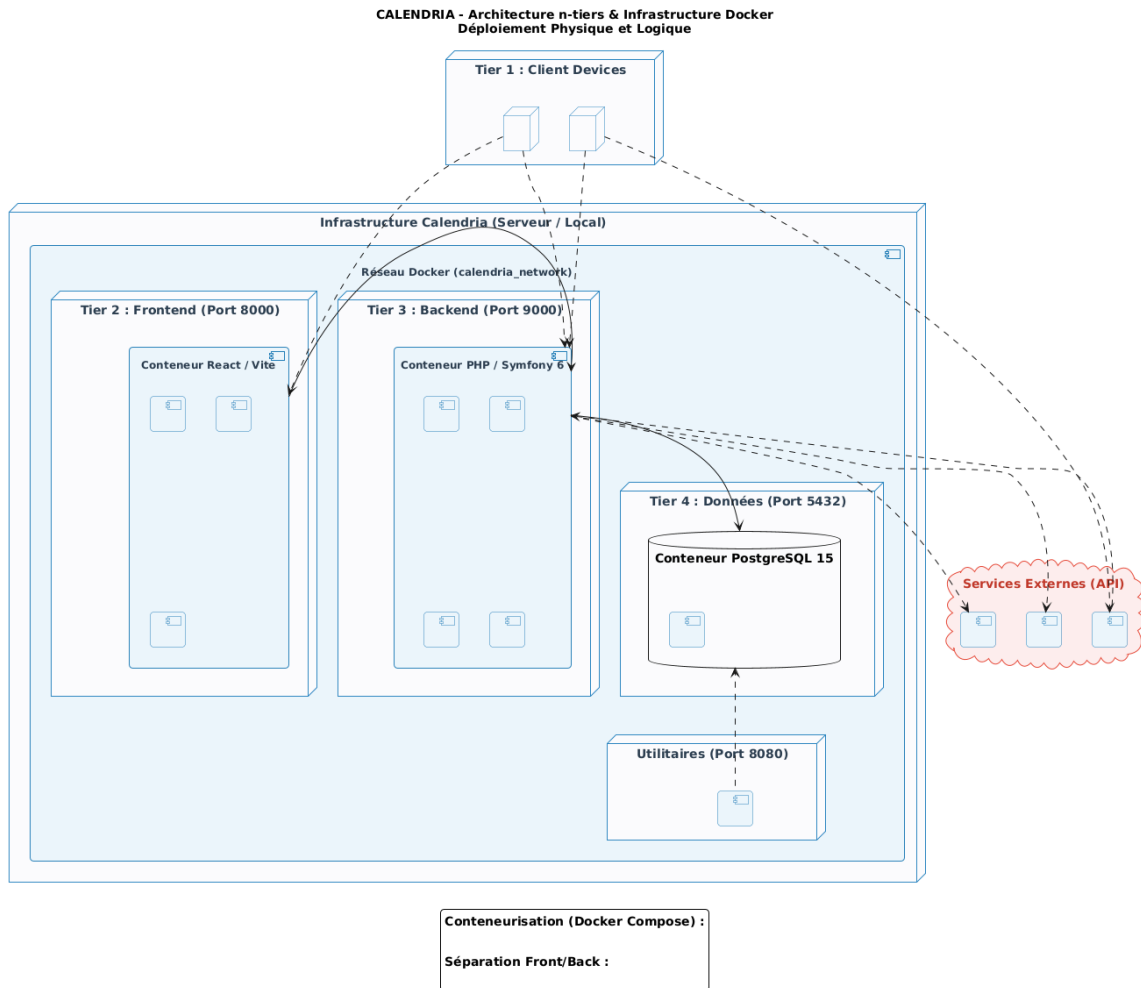
Figure 8.1 - Architecture N-Tiers de CALENDRIA
