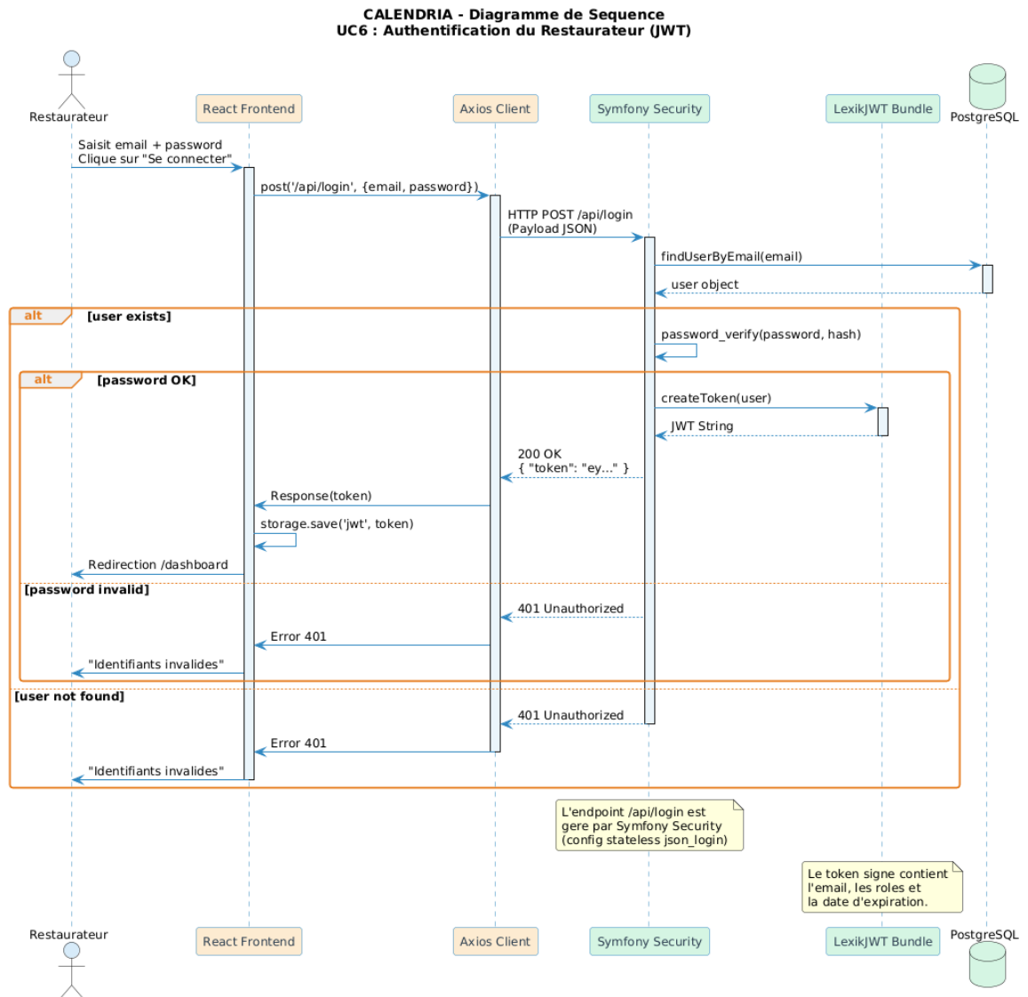
Figure 7.3 - Séquence Authentification JWT
