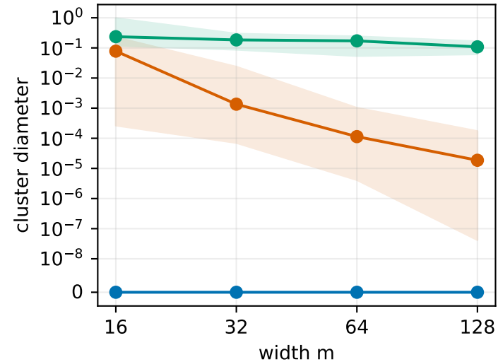
(a) selected cluster geometry
