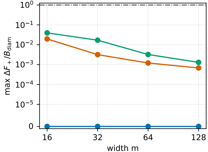
(c) exact-certificate ratio
