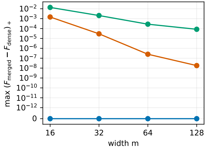
(b) worst merge increment
