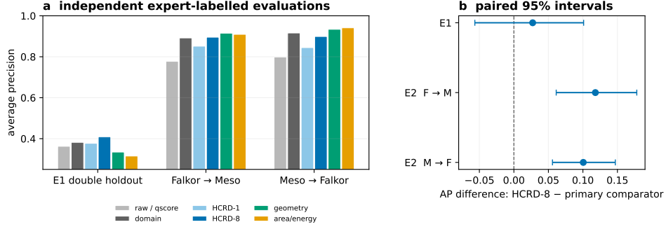
Figure 4: Independent expert-labelled LC-MS evidence. Panel a shows average precision for the first double holdout and both no-refit E2 transfers; “raw / qscore” denotes the task-appropriate minimal representation. Panel b shows the predeclared HCRD-8 difference from the primary comparator. The E1 interval resamples both sample and candidate-ion groups; E2 target-feature intervals are conditional on the trained source models. F and M abbreviate Falkor and MESOSCOPE.
