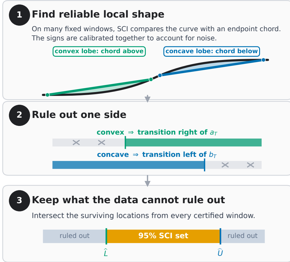
Figure 1: A plain-language overview of SCI. (1) Endpoint chords create signed local residual lobes: the chord is above a convex segment and below a concave segment. The implementation averages these residuals and calibrates all fixed windows together. (2) Certified convexity rules out transition locations on the left, while certified concavity rules out locations on the right. (3) Intersecting all surviving locations gives the SCI confidence set. This schematic illustrates the inversion logic; it is not a substitute for the coverage proof.
