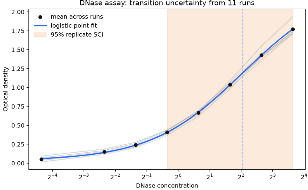
Figure 4: DNase run means, replicate mean curve, descriptive logistic midpoint, and the 95% replicate-curve SCI. Dependence across concentrations inside a run is allowed.
