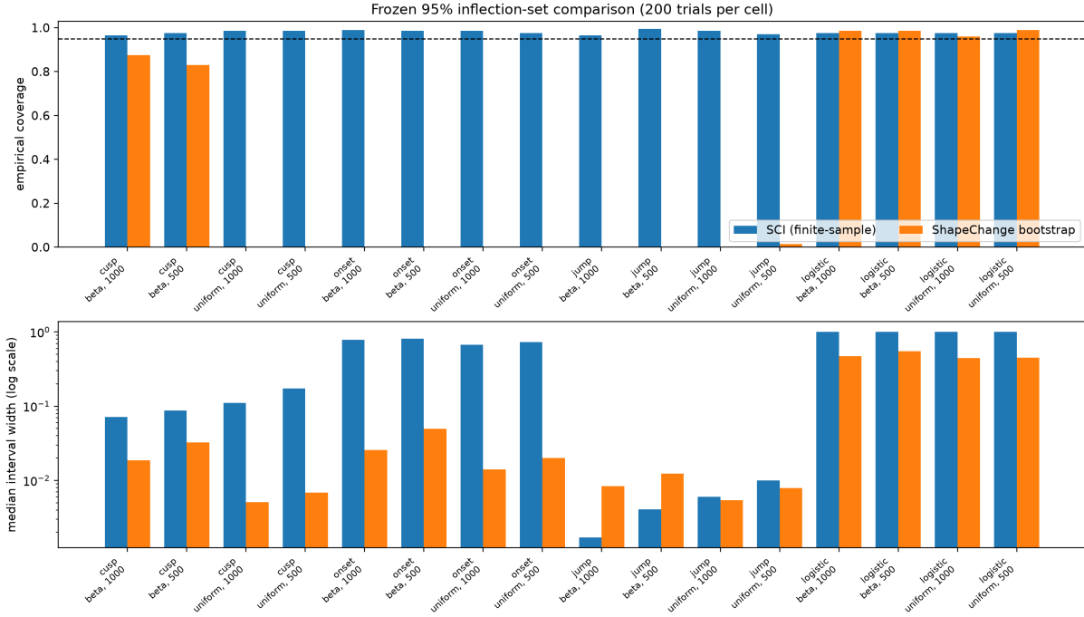
Figure 1: Coverage and width in the initial comparison. The smooth-bootstrap comparator is used inside and outside its smooth regime to expose the practical robustness gap; the comparison does not contradict its published assumptions.
