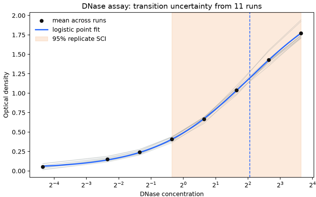
Figure 3: DNase run means, replicate mean curve, descriptive logistic midpoint, and the 95% replicate-curve SCI set. Dependence across concentrations inside a run is allowed.
