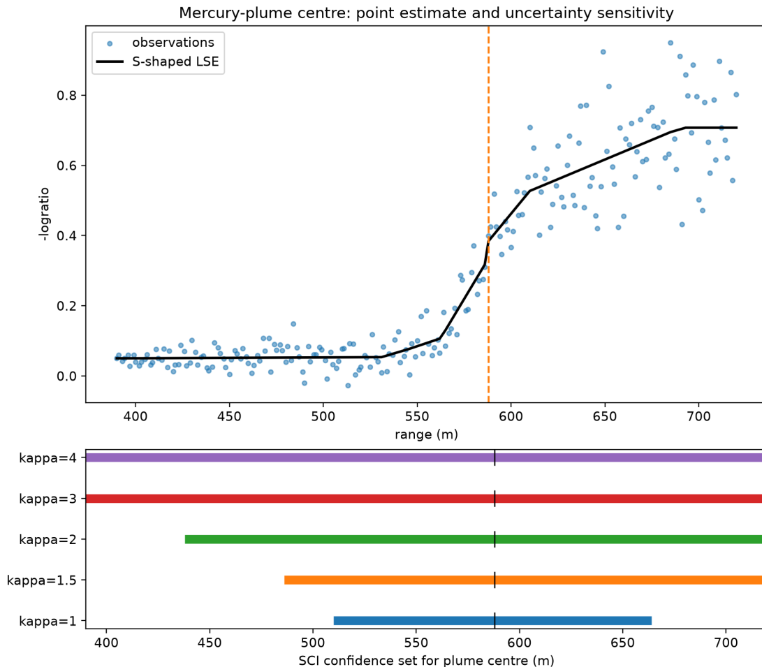
Figure 2: LIDAR transition sets under the declared variance-ratio bound \kappa . Larger heterogeneity allowances produce wider honest sets.
