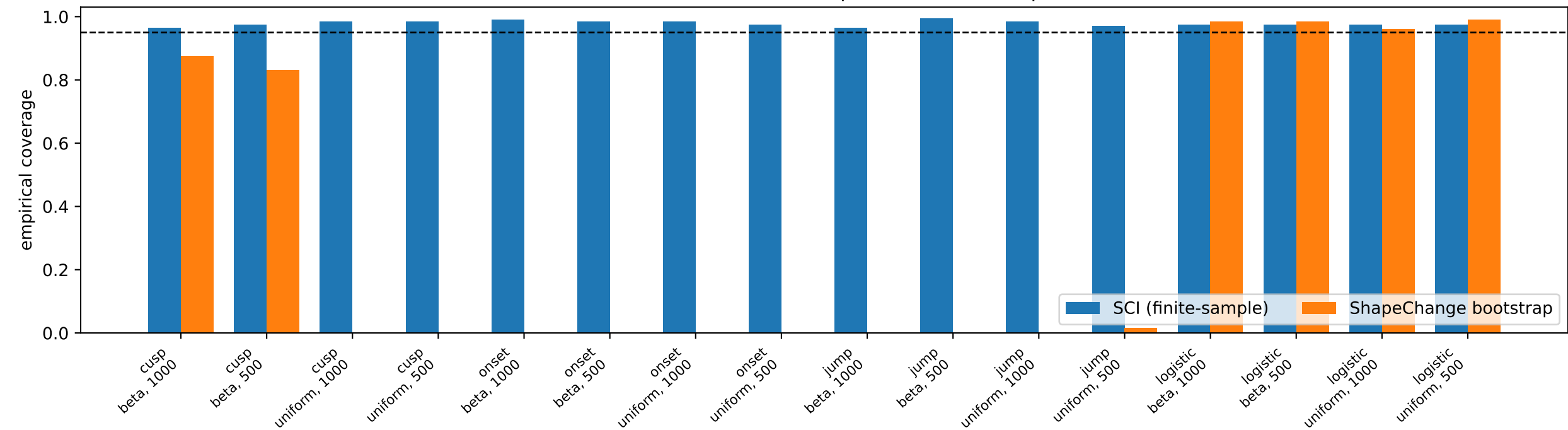
Frozen 95% inflection-set comparison (200 trials per cell)
