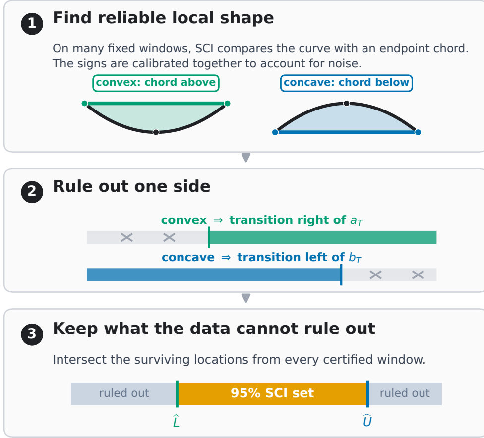
Figure 1: A plain-language overview of SCI. (1) Endpoint chords provide local evidence for convexity or concavity; the implementation averages these residuals and calibrates all fixed windows together. (2) Certified convexity rules out transition locations on the left, while certified concavity rules out locations on the right. (3) Intersecting all surviving locations gives the SCI confidence set. This schematic illustrates the inversion logic; it is not a substitute for the coverage proof.
