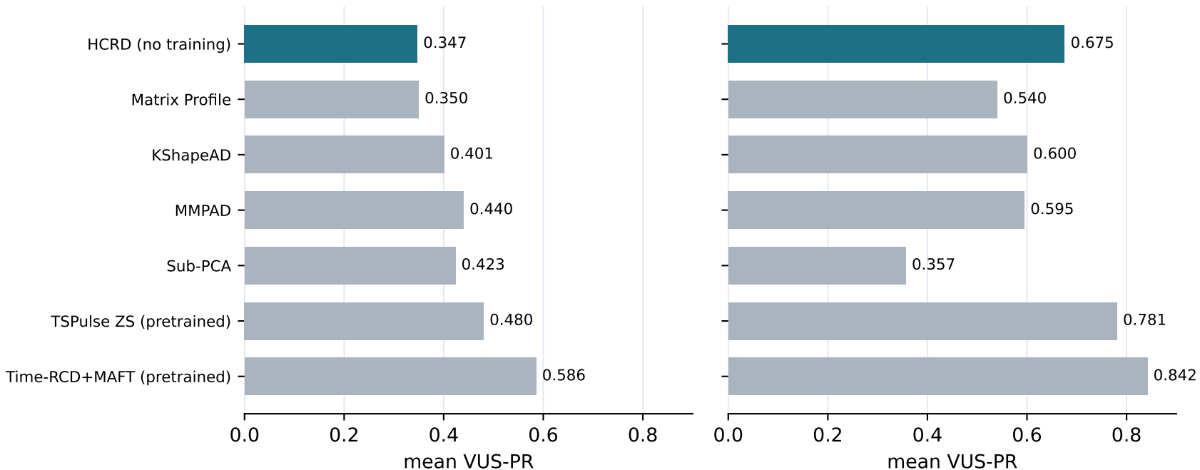
49 point-anomaly series
