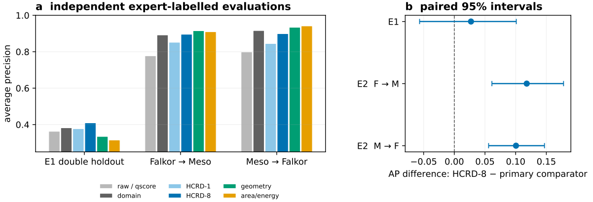
Figure 2: Independent expert-labelled LC-MS evidence. Panel a shows average precision for the first double holdout and both no-refit E2 transfers; “raw / qscore” denotes the task-appropriate minimal representation. Panel b shows the predeclared HCRD-8 difference from the primary comparator. The E1 interval resamples both sample and candidate-ion groups; E2 intervals are paired feature bootstraps. F and M abbreviate Falkor and MESOSCOPE.
