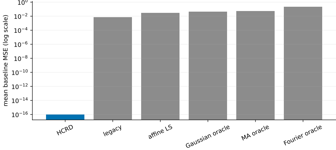
Figure 3: Baseline error on the theorem-matched noiseless class. Centred HCRD recovers the baseline to machine precision; thresholded HCRD and an endpoint-only RDP solution tie it numerically and are therefore not labelled as strictly inferior.
