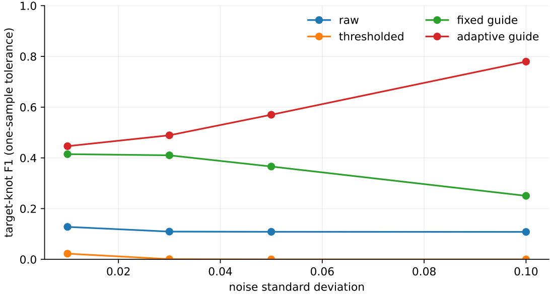
Figure 4: Knot accuracy under repeated Gaussian perturbations. Stability alone is insufficient: the thresholded method is stable because it often retains only endpoints, whereas adaptive guidance retains a compact set of meaningful knots.
