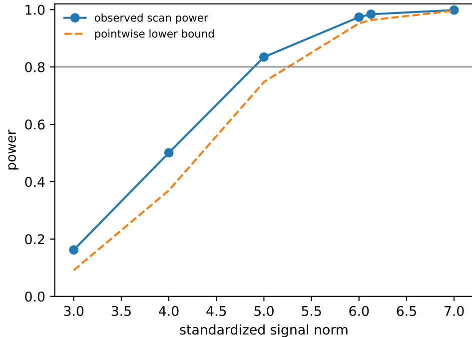
Finite-sieve power
