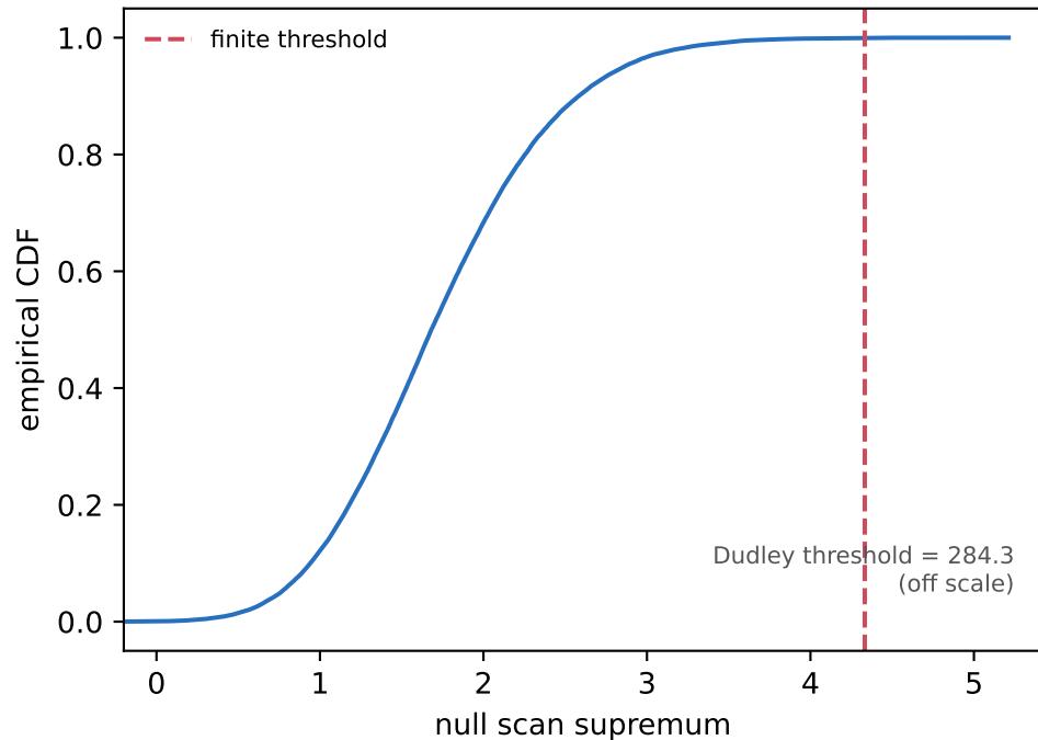
Null calibration
