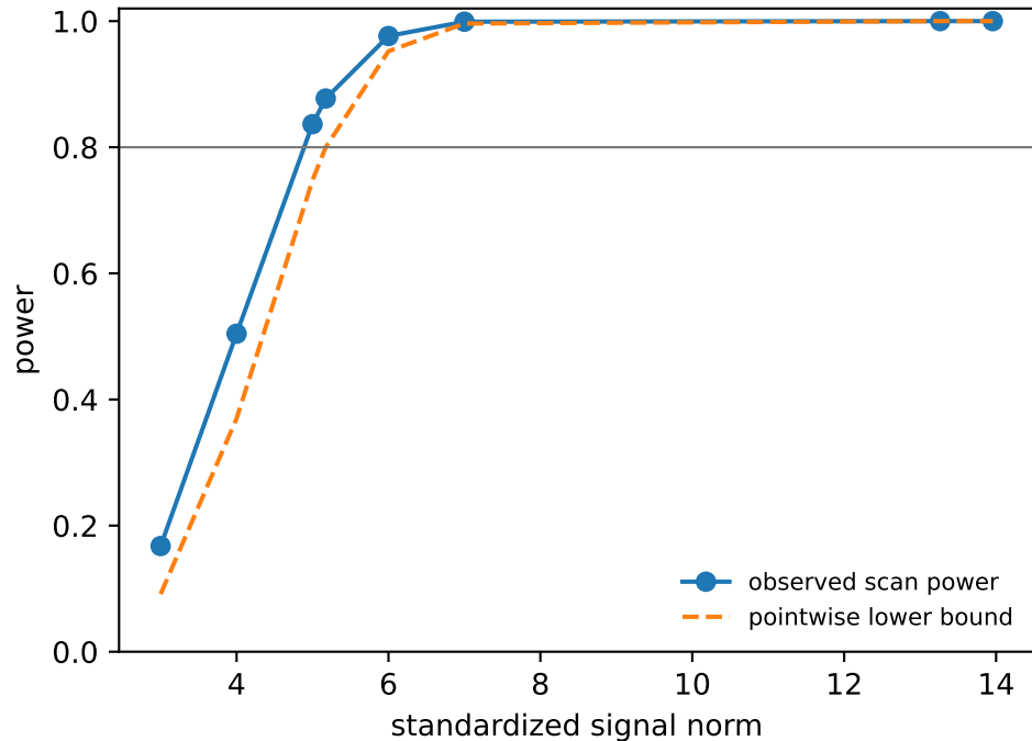
Finite-sieve power
