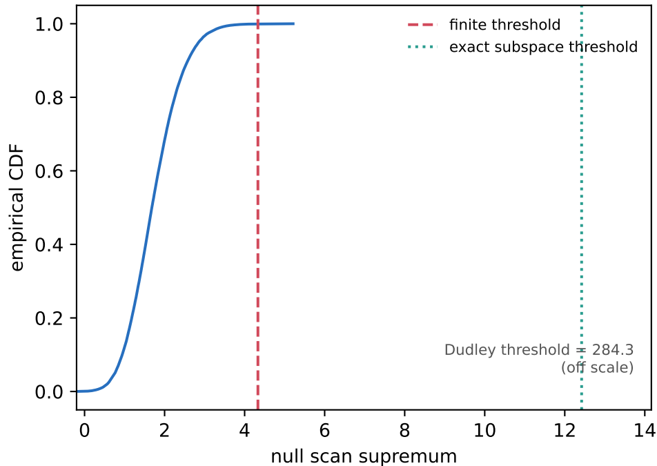
Null calibration
