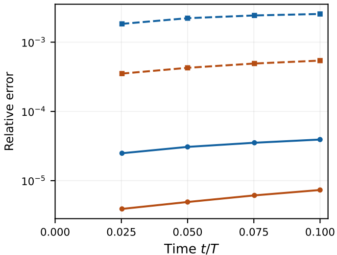
Wave-normalised surface error
