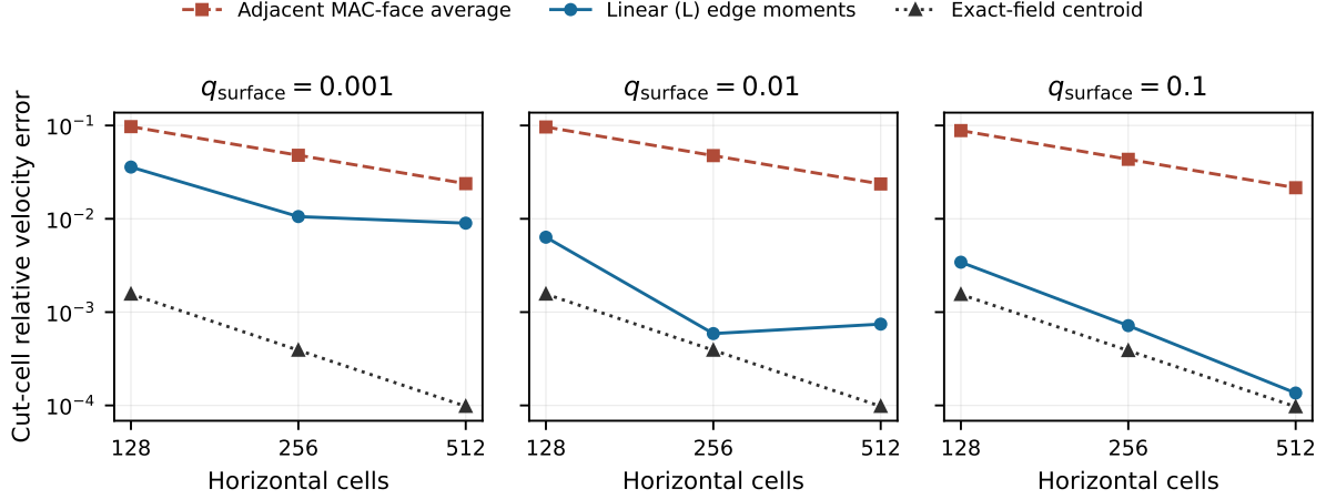
Figure 4: Flat-boundary stress tests before native projection. The prescribed surface fraction is shown above each panel; the error norm includes both cut rows. The L reconstruction improves on adjacent-face averaging, but the exact-field centroid control is more accurate in all nine cases.
