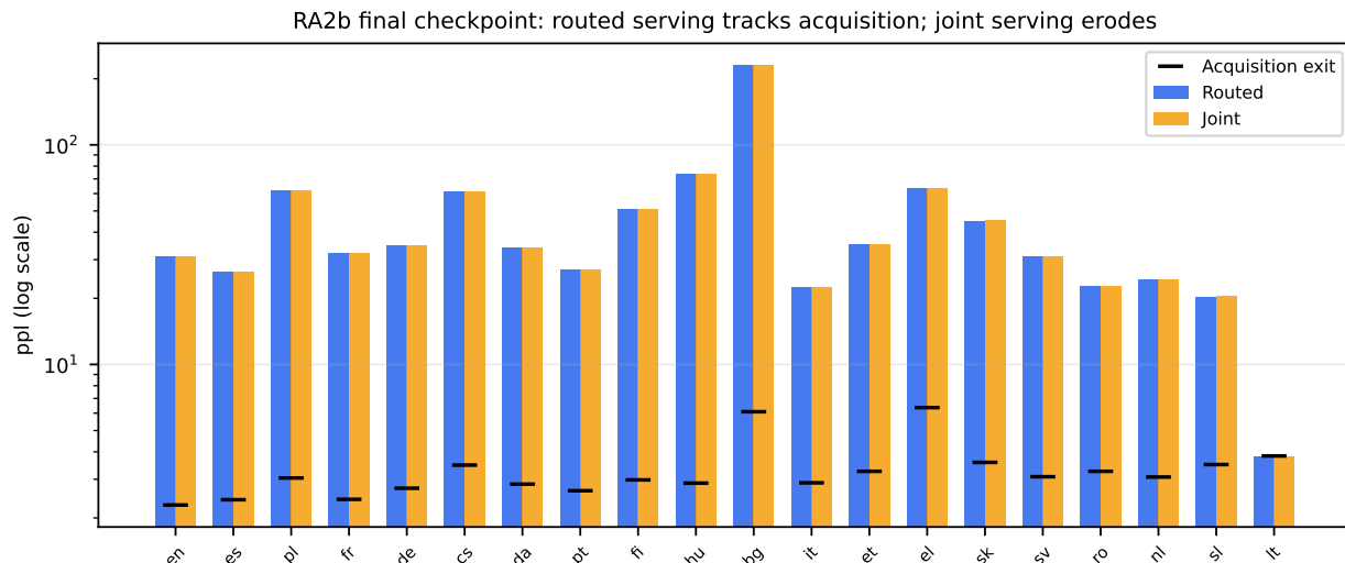
Figure 3: RA2b final checkpoint: routed serving (blue) vs joint serving (orange) vs acquisition exit (black tick), per domain, log scale. Routed tracks acquisition for every domain (median +4.3% over the acquisition exit, range -0.8\% to +8.0\% , worst case hu); joint serving erodes 1.0\text{--}37.8\times (median 11\times ) — the interference term that survives the fix. Sources: docs/reports/data/a4_offset_band/ and readout §B4.
