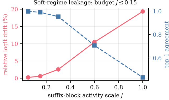
Figure 3: Measured soft-regime leakage from a suffix block into old-language serving. Relative logit drift and top-1 agreement vary with suffix-block activity; the hard endpoint remains the only exactly measured preservation mechanism. This figure is evidence for the scope of the theory, not a replacement for the proof.
