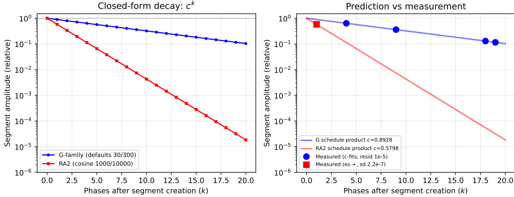
Figure 2: Optimizer decay regimes used to audit the confound. The closed-form schedule product predicts the measured per-segment scale factors; the RA2 and default schedules differ in the resulting decay rate.
