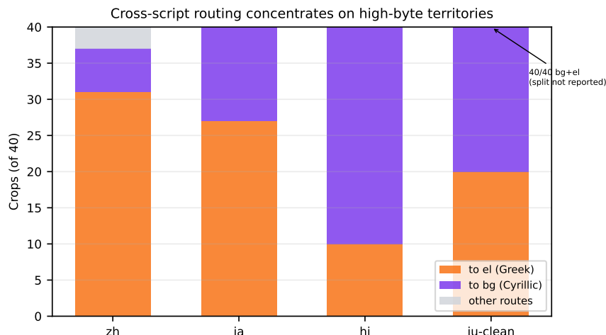
Figure 9: Cross-script routing on the fixed-regime chain (40 crops per probe). zh 37/40, ja 40/40, hi 40/40 and the decontaminated iu 40/40 concentrate on the only two territories with substantial multi-byte training exposure (bg/el: 82% 2-byte characters vs 11.7% next-highest); no Latin-route attraction remains after the iu correction. No linguistic kinship exists between any probe and Cyrillic or Greek.
