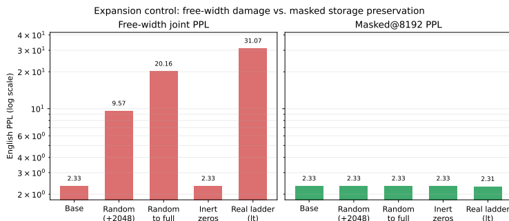
Figure 7: Expansion control on the English-era base. The left panel reports free-width joint PPL and the right panel reports masked PPL at the original width. Random untrained growth reaches 9.57 after one block and 20.16 at full width; inert zeros remain at 2.33; the real ladder reaches 31.07 free but 2.31 masked. Thus the real growth arm is shown explicitly in both serving regimes, separating arithmetic readout damage from storage preservation.
