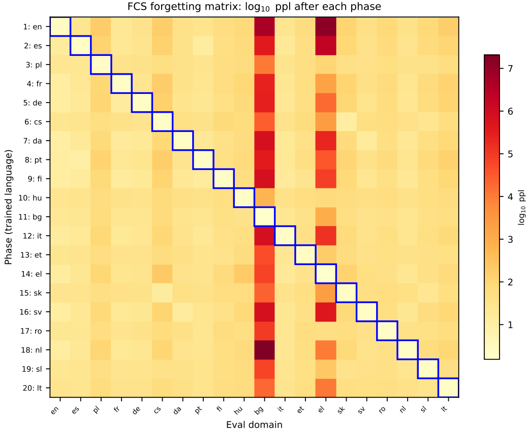
Figure 4: FCS forgetting matrix ( \log_{10} ppl). Each row is the 20-domain cold eval after that phase; blue box marks the diagonal. Latin-script languages fall to their English-only zero-shot level (nine of the sixteen zero-shot-comparable domains fully displaced, seven partial retention; en, lt, bg, el excluded); bg/el collapse by up to four orders of magnitude at row 20 ( \text{bg} \times 12,086 , \text{el} \times 6,873 relative to acquisition); family-structured oscillation survives throughout.
