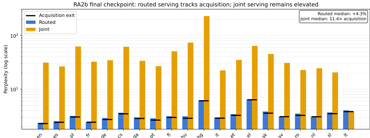
Figure 6: RA2b final checkpoint: routed serving (blue), joint serving (orange), and acquisition exit (black tick), per domain, log scale. Routed serving remains within the measured acquisition-cost band (median +4.3%, range -0.8\% to +8.0\% ; maximum +8.0\% at hu). Joint serving ranges from 1.0\times to 37.8\times acquisition (median 11.4\times ). Values are regenerated from the committed A4 routed-cost table and the final RA2b matrix.
