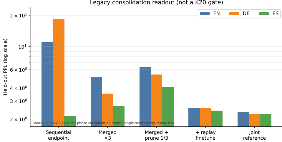
Figure 10: Legacy consolidation readout. Merge, random pruning, and brief replay approach the joint reference for EN/DE/ES in the historical three-phase experiment. This is contextual evidence for consolidation, not evidence for the K20 routing, storage, or readout gates.
