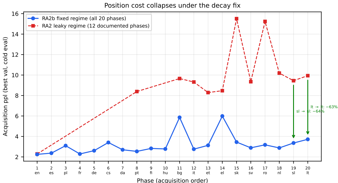
Figure 5: Ladder acquisition. RA2b (fixed regime, blue, all 20 phases): 2.25–5.99 band, position cost gone. RA2 (leaky regime, red, 12 documented phases): acquisition tracked ladder position. Green arrows: same-position same-host cells lt 9.94 \rightarrow 3.72 (–63%), sl 9.45 \rightarrow 3.36 (–64%). Residual spread is alphabet difficulty (bg/el), not chain state.
