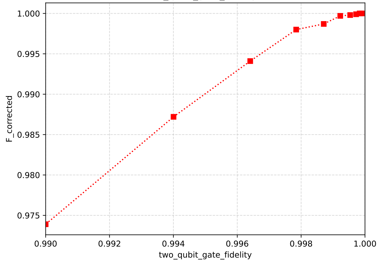
linear scale (two_qubit_gate_fidelity in [0.99, 1.0])
