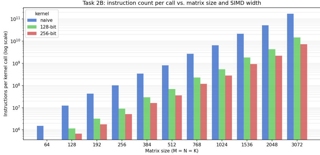
Figure 7: Instructions executed per kernel call vs. matrix size ( M=N=K ), for matmul_naive , the 128-bit SIMD kernel, and the 256-bit (AVX2) kernel. Per-call figures are the per-symbol instruction count from perf record (event_count × overhead %) divided by the number of times the harness invokes each kernel in a single-stage run (naive: 6, SIMD: 5). Log scale.
