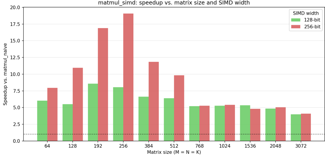
Figure 8: Speedup of matmul_simd over matmul_naive vs. matrix size ( M=N=K ), for the 128-bit and 256-bit SIMD kernels.
