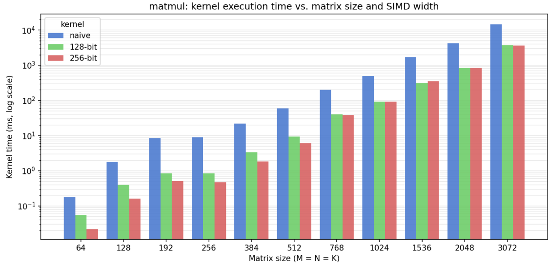
Figure 9: Kernel execution time (ms, log scale) vs. matrix size ( M=N=K ). Same runs as Fig. 8.
