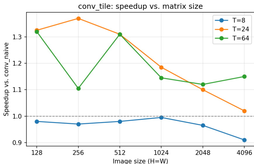
Figure 6: Speedup vs. matrix size, one line per tile size.
