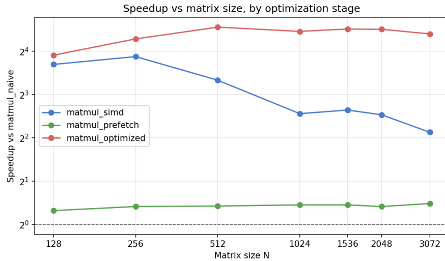
Figure 10: Speedup of matmul_simd , matmul_prefetch , and matmul_optimized over matmul_naive vs. matrix size (log-log).
