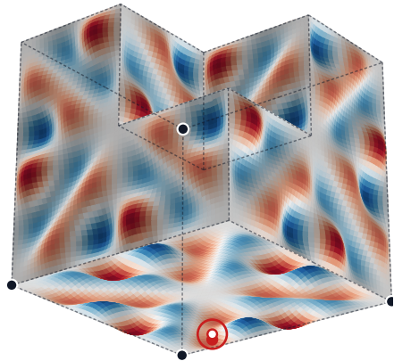
C: k = (\frac{3}{2}, \frac{3}{2}, 1) , e = (1, 0, 0)
