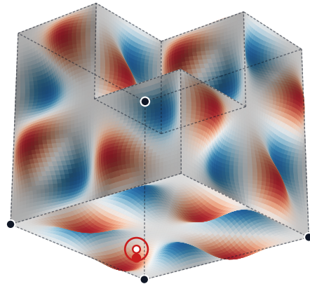
A: k = (1, \frac{1}{2}, \frac{1}{2}) , e = (1, 1, 0)
