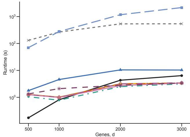
Runtime across gene dimensions (n = 2,000)
