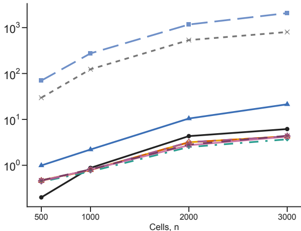
Runtime across cell numbers (d = 2,000)
