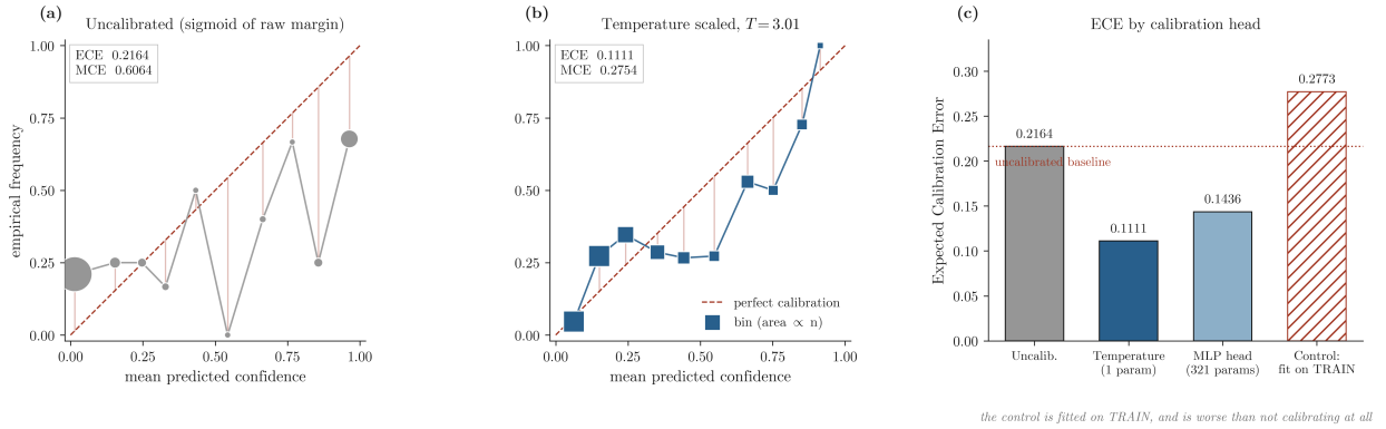
Figure 4: Reliability before and after temperature scaling, with the train-fitted leakage control at right. Bin values are read directly from the run artifacts; no curve is fitted.
