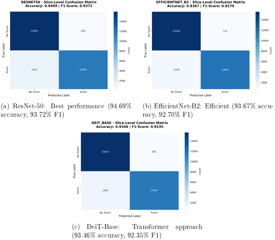
Figure 4.2: Confusion matrices for slice-level tumor detection on test set (187 patients, \sim 29,000 slices). All models show balanced performance with high accuracy and F1-scores, demonstrating effective tumor/non-tumor classification.
