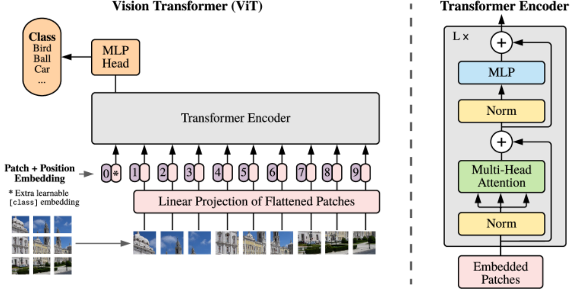
Figure 3.1: Model overview. We split an image into fixed-size patches, linearly embed each of them, add position embeddings, and feed the resulting sequence of vectors to a standard Transformer encoder. In order to perform classification, we use the standard approach of adding an extra learnable “classification token” to the sequence. The illustration of the Transformer encoder was inspired by Vaswani et al. (2017).
