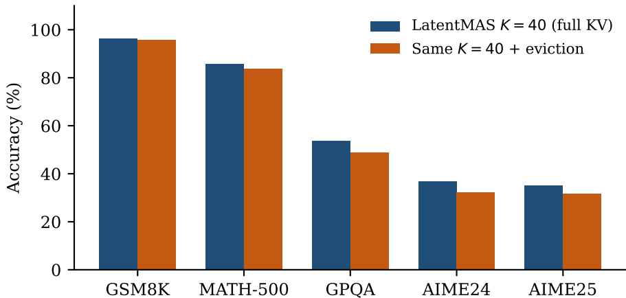
Eviction after a K = 40 rollout (3-seed mean; AIME25: 2 seeds)
