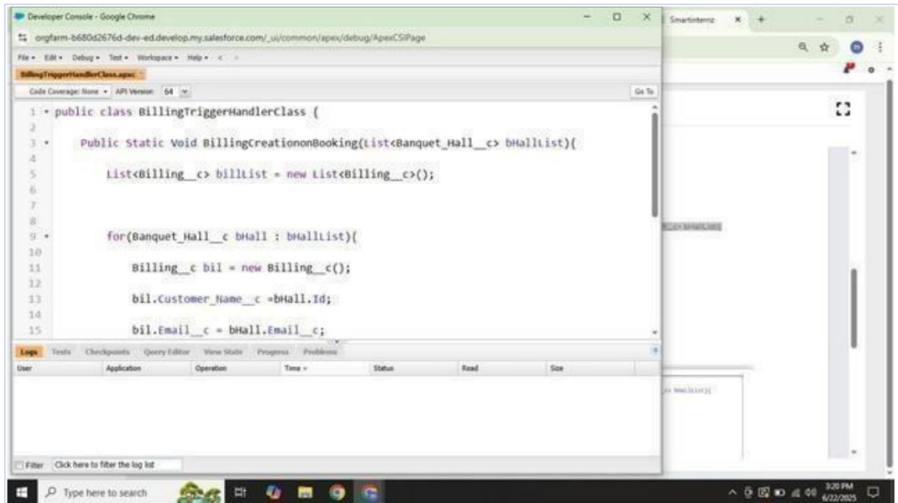
Figure 15: BillingTriggerHandlerClass in the Developer Console
