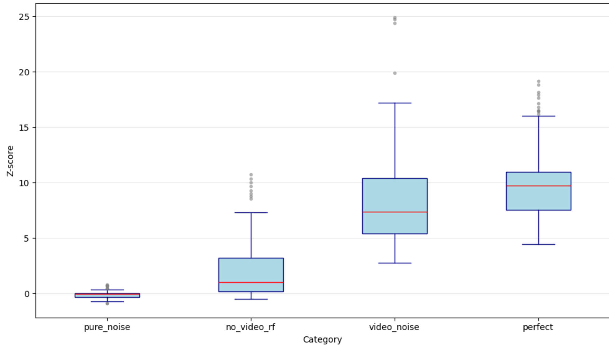
Autocorrelation masked z-score distribution
