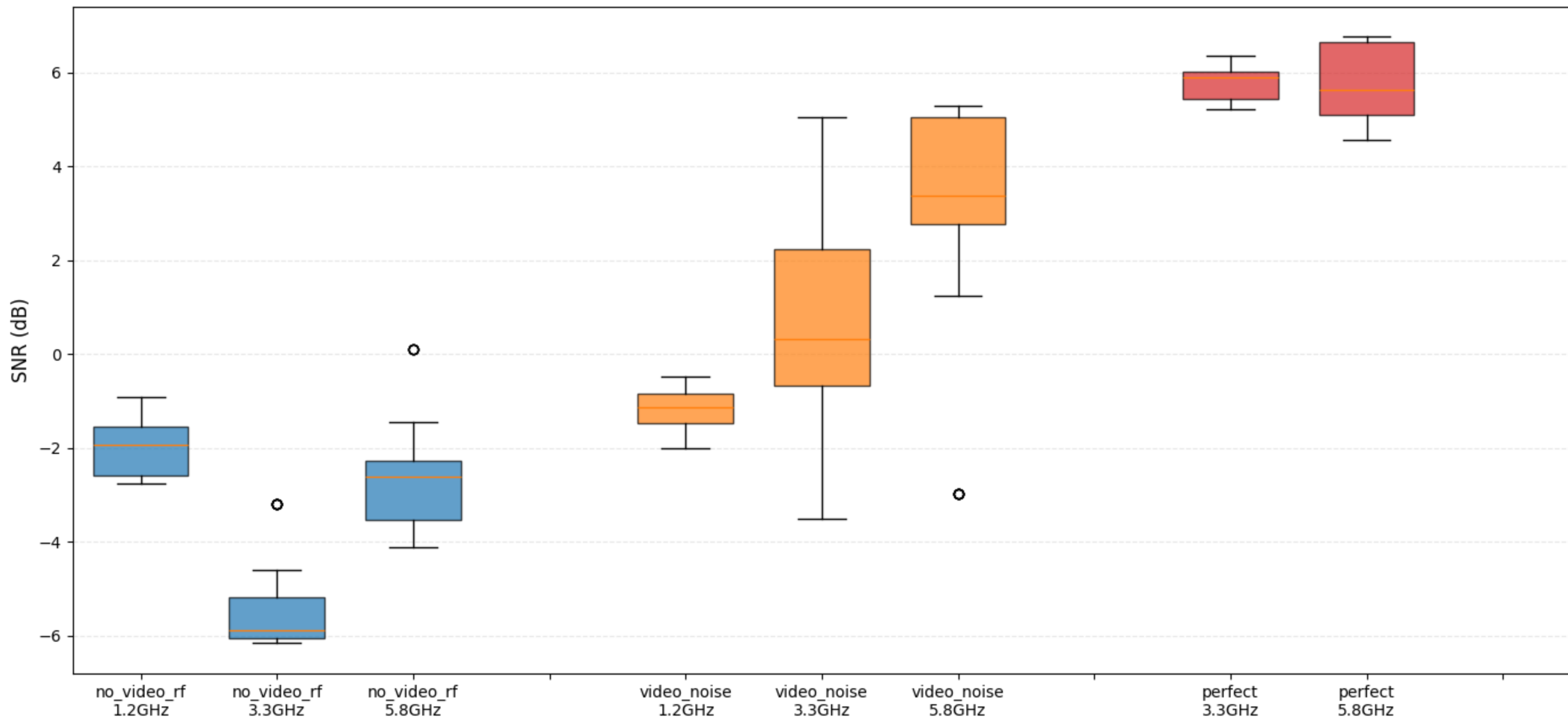
SNR Distribution Grouped by Signal Quality
