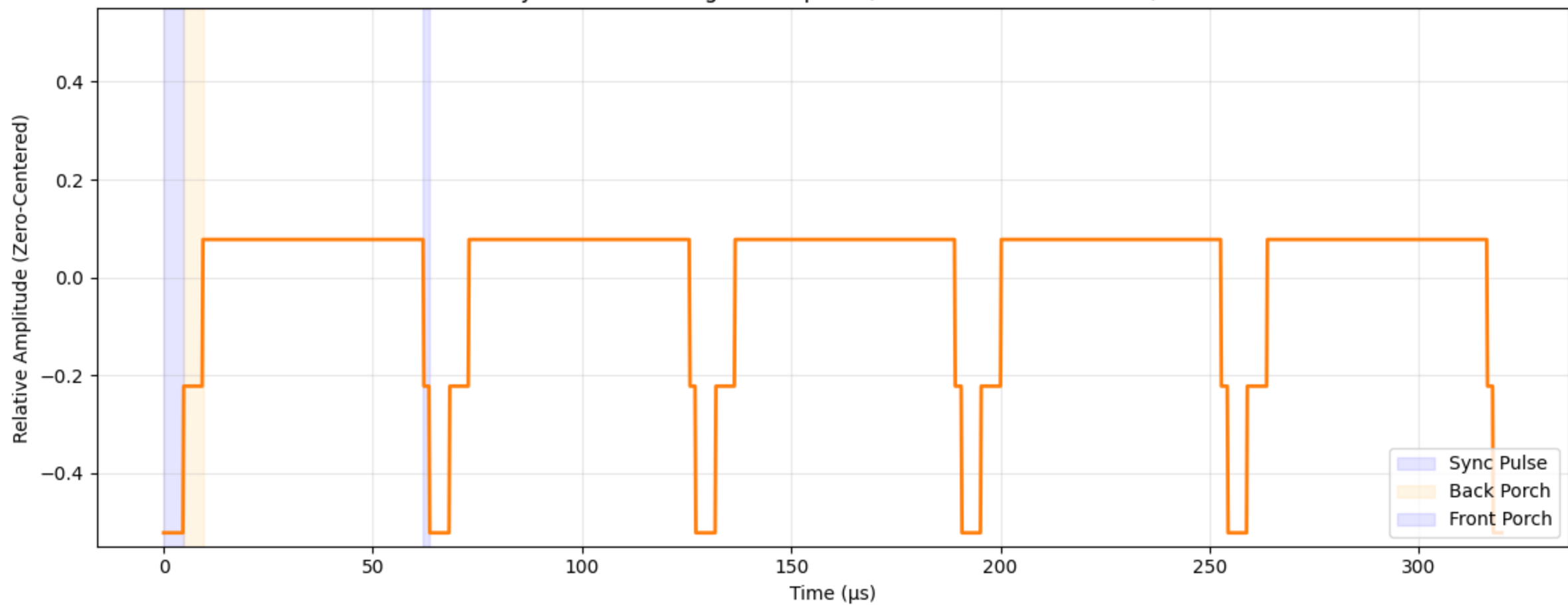
Synthetic NTSC Signal Template (Matched Filter Reference)
