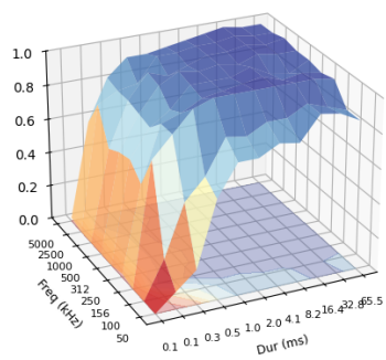
Method: MATCHED (Sensitivity)
