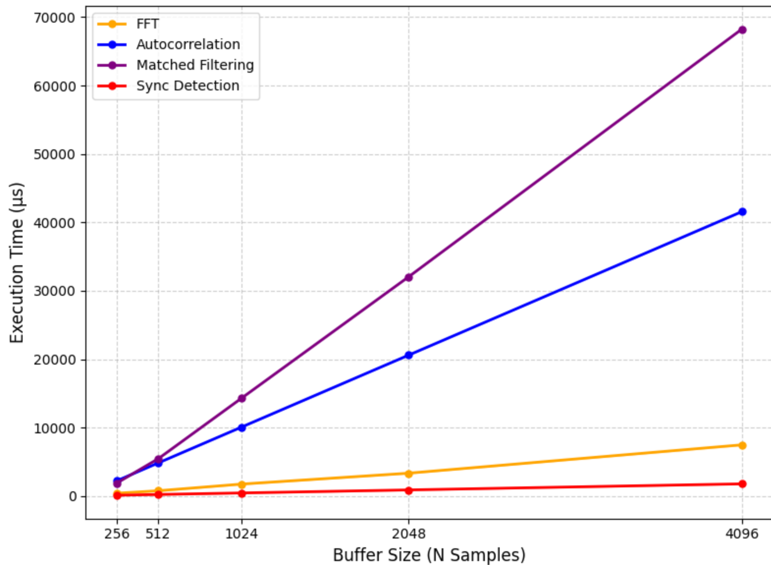
Board Performance: STM32F411E-DISCOVERY
