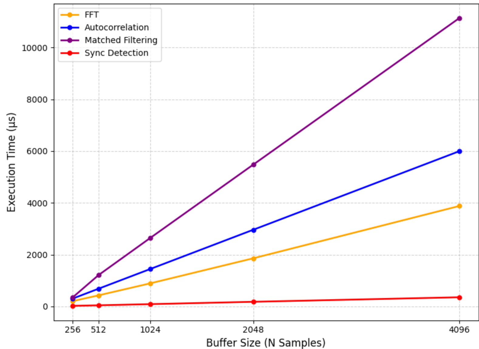
Board Performance: ESP32-WROOM-32E
