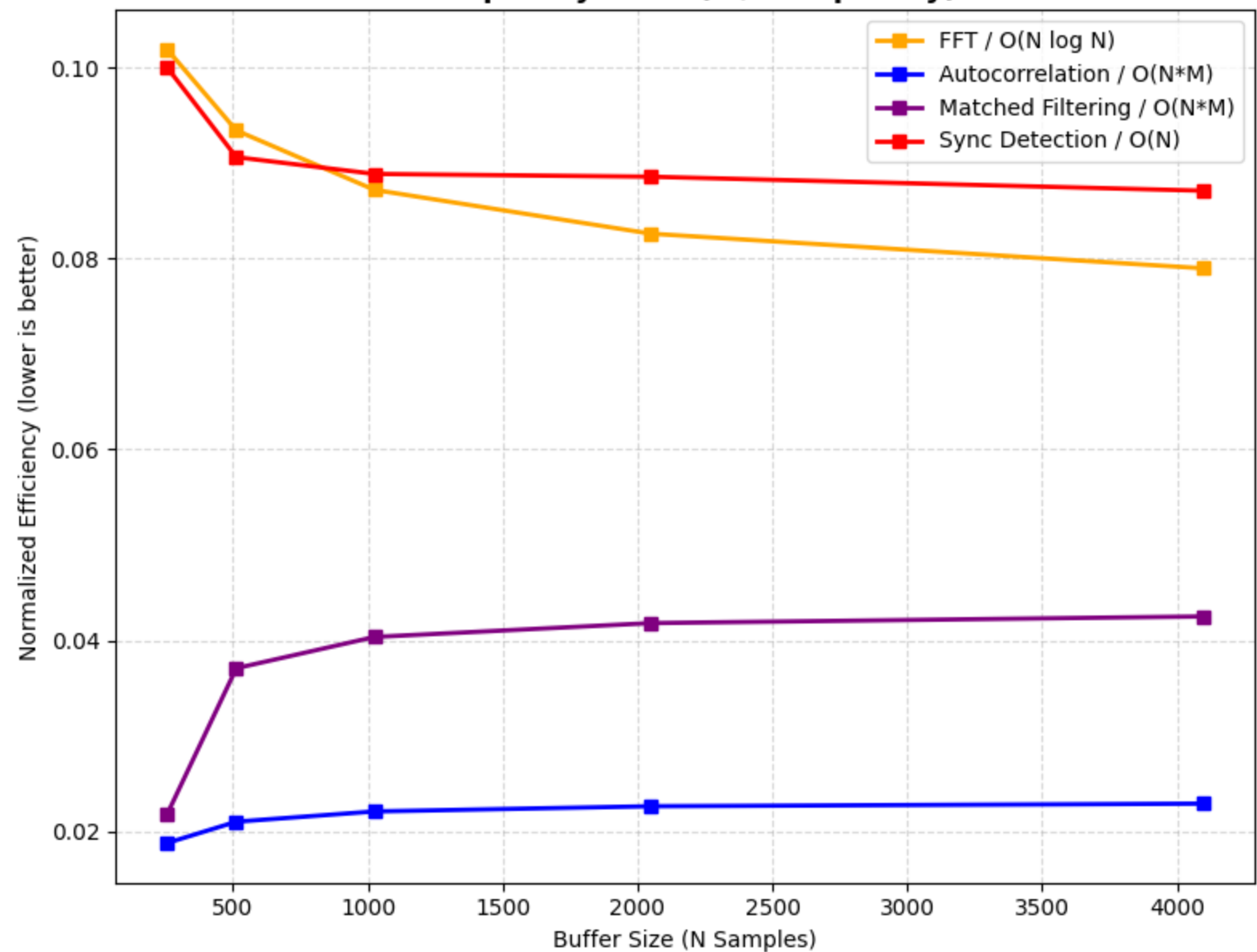
Complexity Ratio (T / Complexity)
