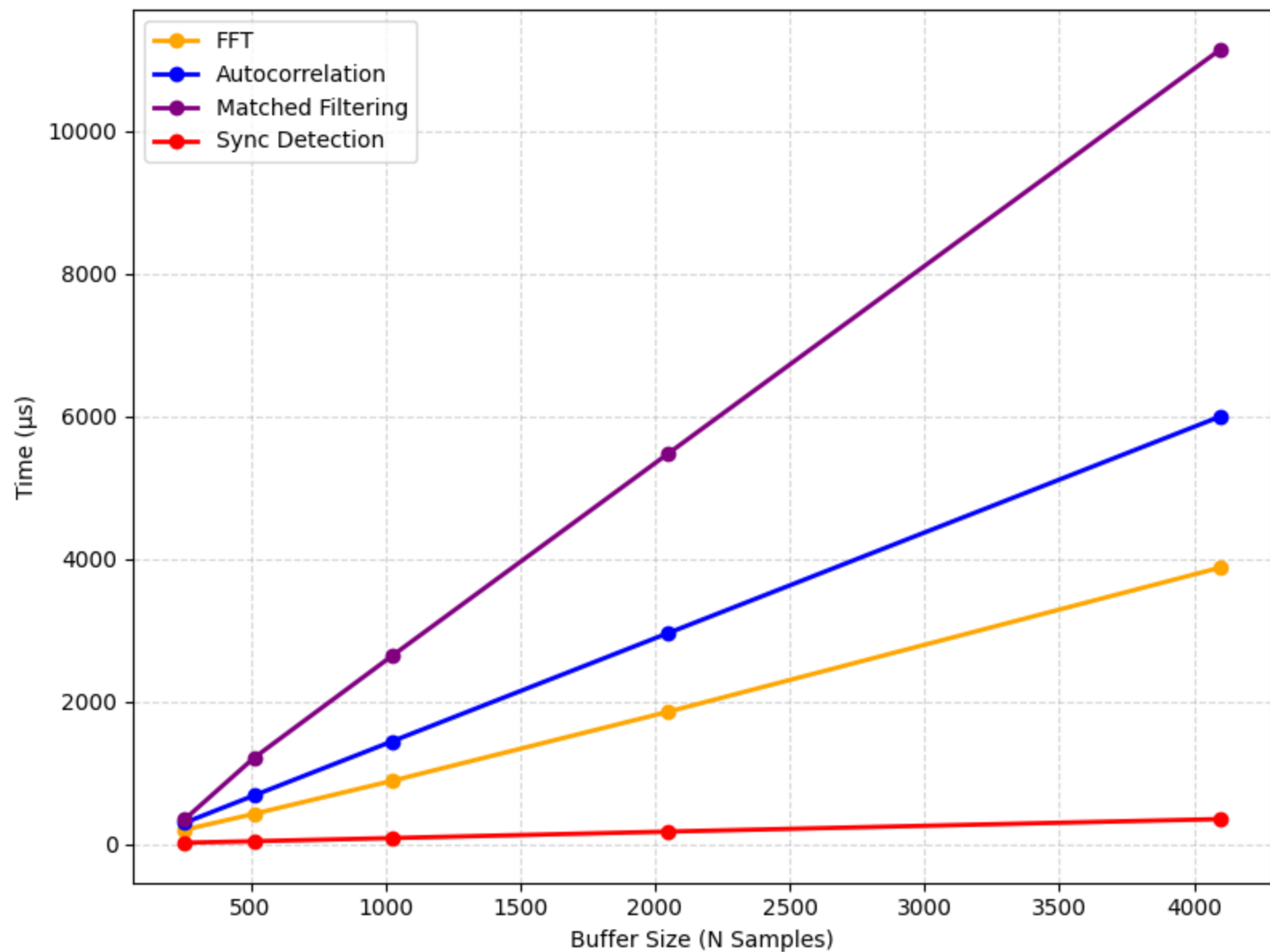
Raw Execution Time Board: ESP32-WROOM-32E
