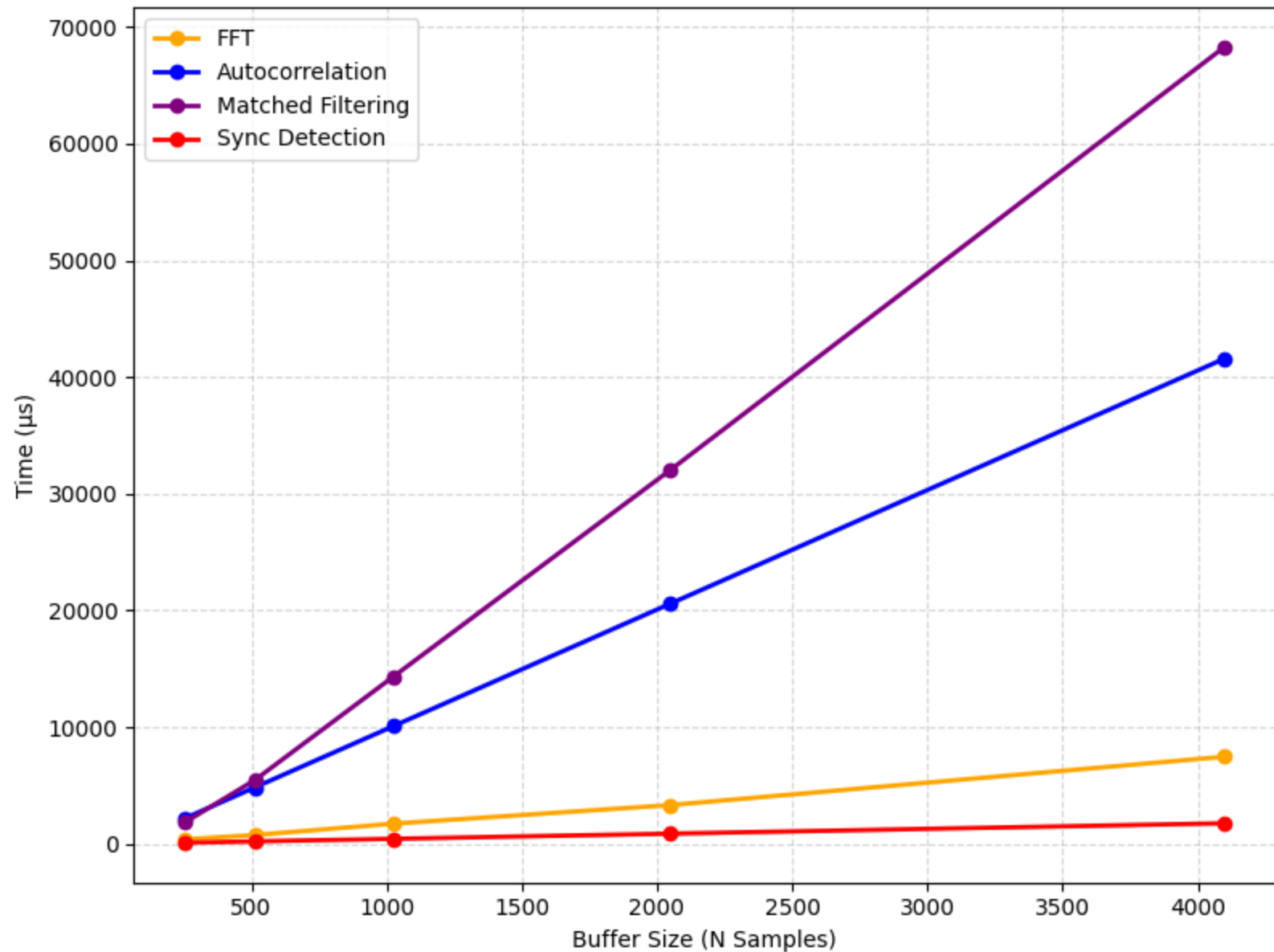
Raw Execution Time Board: STM32F411E-DISCOVERY
