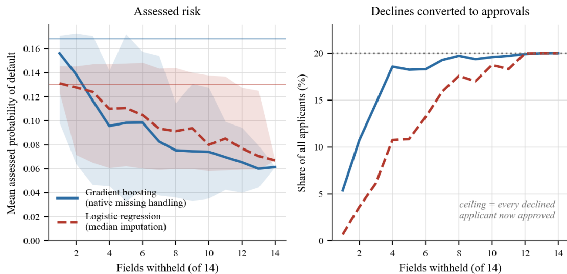
Figure 5.9: The effect of withholding information about the same applicants. Left: mean assessed probability of default as fields are withheld, shaded across draws, with the thin horizontal line marking each model's assessment when nothing is withheld. Right: the share of all applicants converted from decline to approval. Both models converge on the ceiling, at which every applicant who would have been declined is approved.
