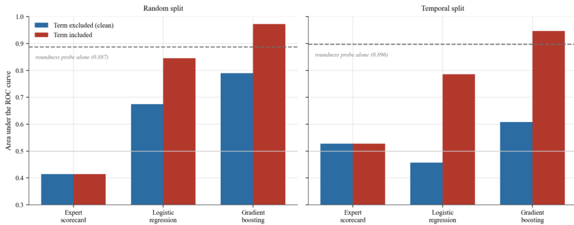
Figure 5.4: Discrimination with and without the *Term* field, under both validation protocols. The dashed line marks the level the roundness boolean reaches on its own.
