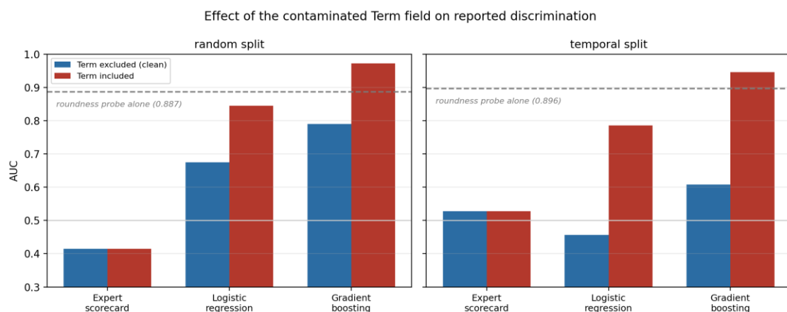
Figure 5.4: Discrimination with and without the Term field under both validation protocols. The dashed line marks the AUC reached by the roundness boolean alone.
