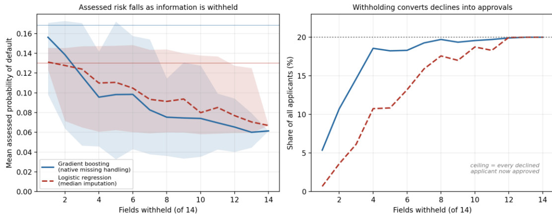
Figure 5.7: Effect of withholding information on the same applicants. Left: mean assessed probability of default as fields are withheld, shaded across draws. Right: the share of all applicants converted from decline to approval. Both models converge on the ceiling, at which every applicant who would have been declined is approved.
