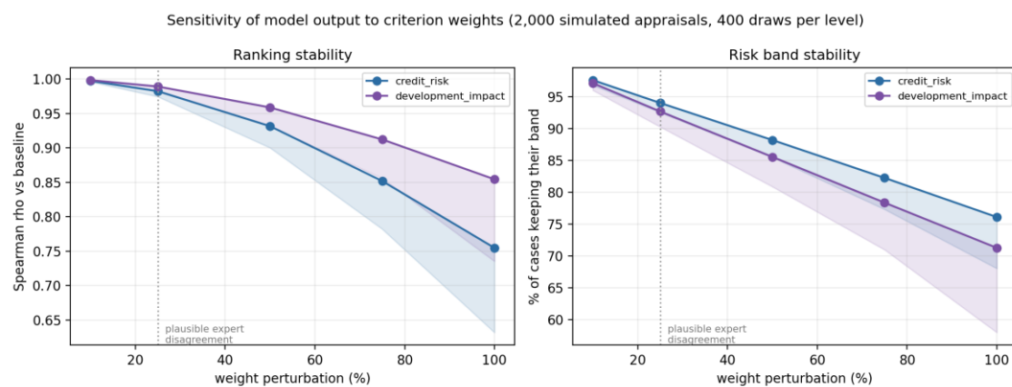
Figure 5.6: Ranking stability and risk-band stability against the magnitude of weight perturbation. Shaded bands show the range down to the 5th percentile across draws. The dotted line marks the level of disagreement practitioners plausibly exhibit.
