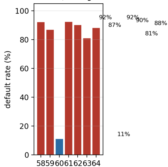
Figure 5.1: Default rate by exact contractual term, 2007 approvals. Terms that are multiples of twelve are shown in blue.
