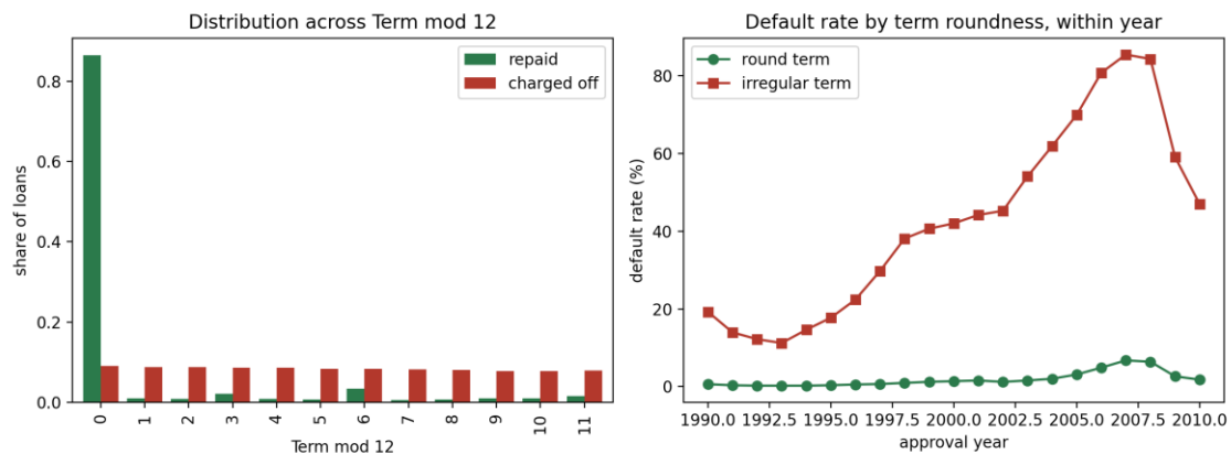
Figure 5.2: Distribution across Term mod 12 (left) and default rate by term roundness within each approval year (right). Repaid facilities cluster at residue zero; charged-off facilities spread almost uniformly.
